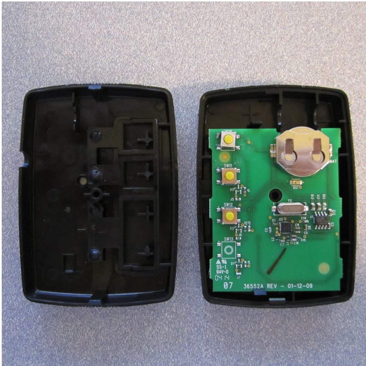
Figure 1: GIDFX3 Internal View / PCB Top
