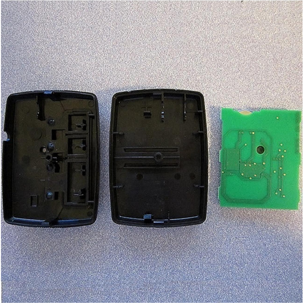
Figure 2: GIDFX3 Internal View / PCB Bottom
