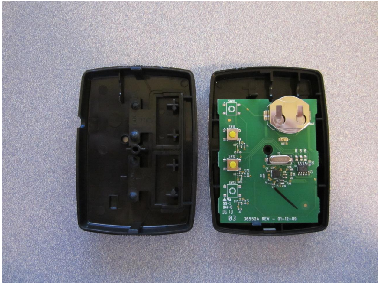
Figure 1: GIDFX2 Internal View / PCB Top
