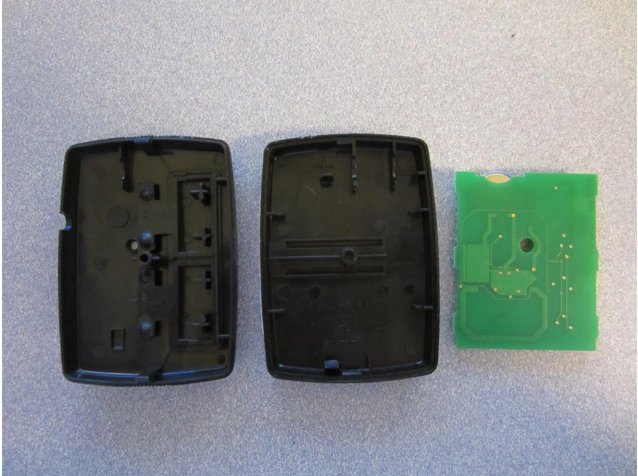
Figure 2: GIDFX2 Internal View / PCB Bottom
