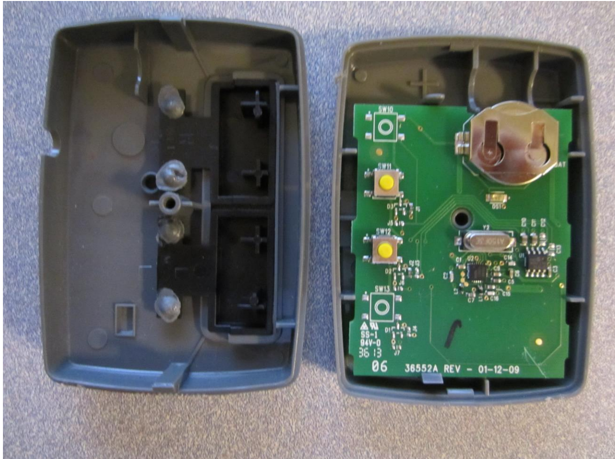
Figure 3: OCDFX2 Internal View / PCB Top
