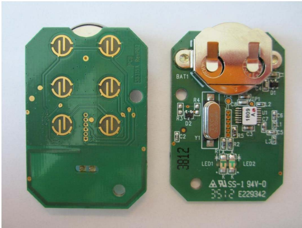
Transmitter PCB Front and Back
