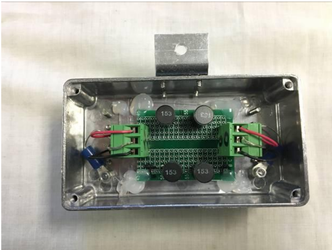
Figure 7. Filter #2 (Passive) with Bottom Cover Removed
