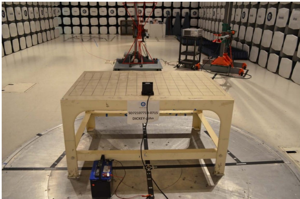
Radiated Emissions Test Setup (30MHz to 1GHz, Back)
