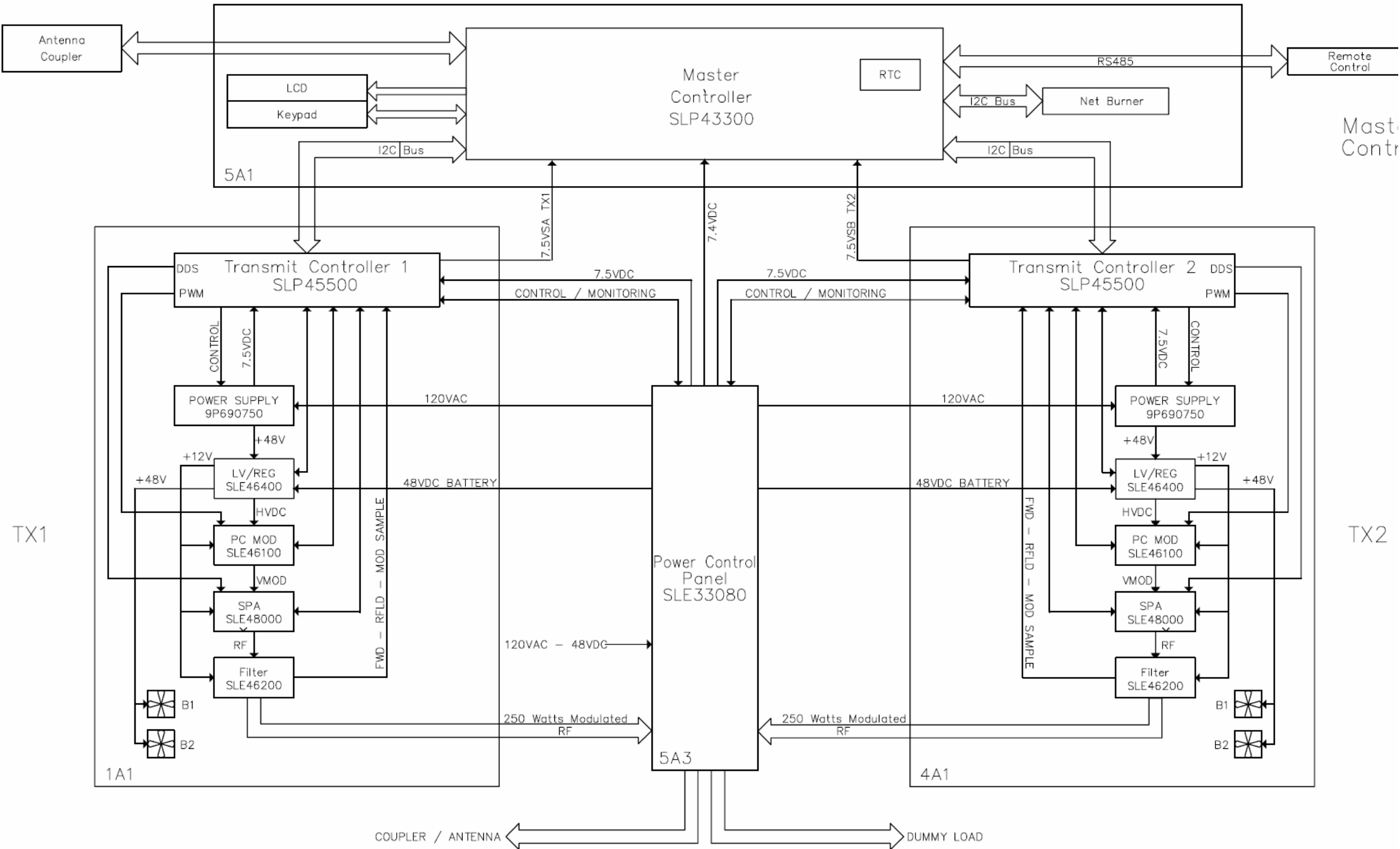
SDB33030 Rev A SE250 – Transmitter Block Diagram
