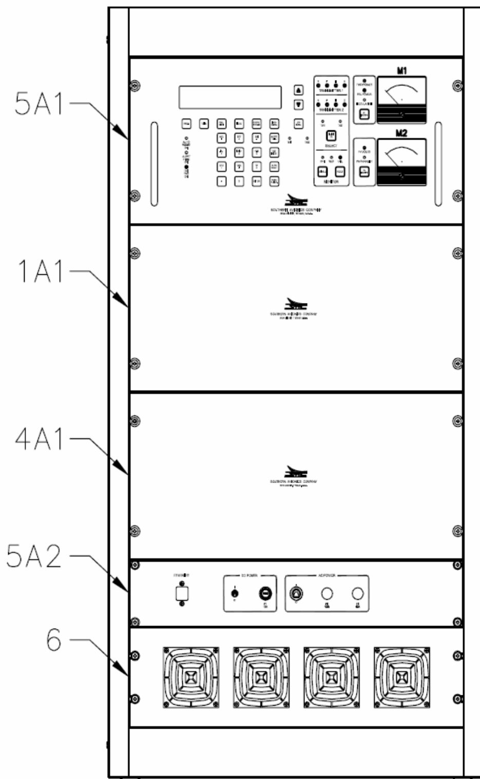
SDF34030 Rev C SE250 Transmitter diagram (front view)
