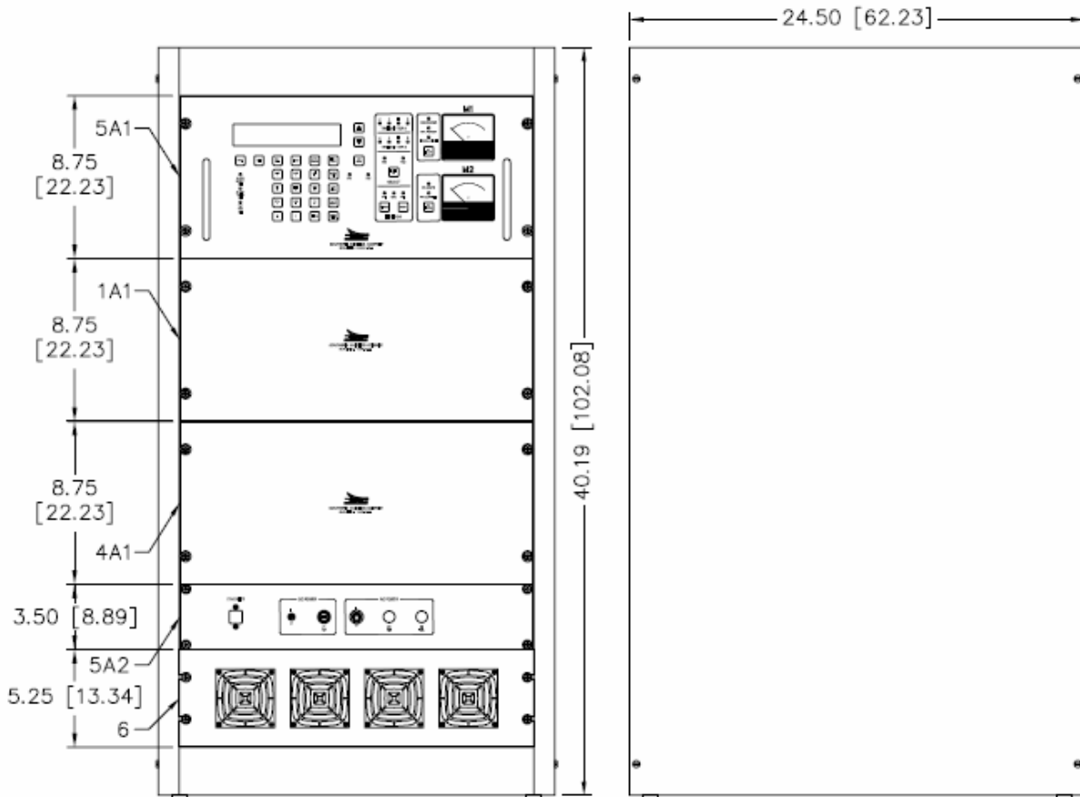
FRONT VIEW
