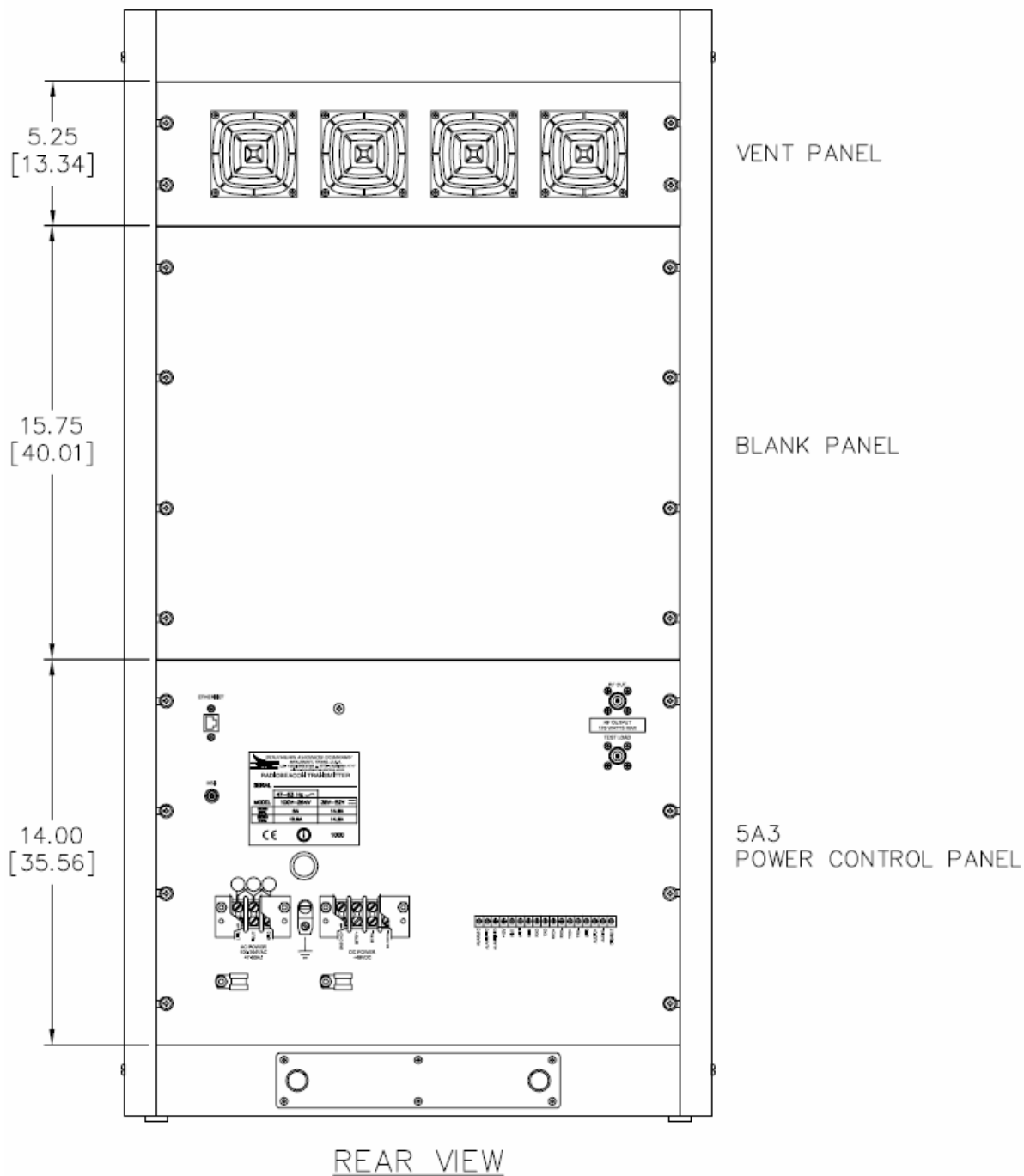
SDF33030 Rev C SE250 Rack mount rear enclosure dimensions
