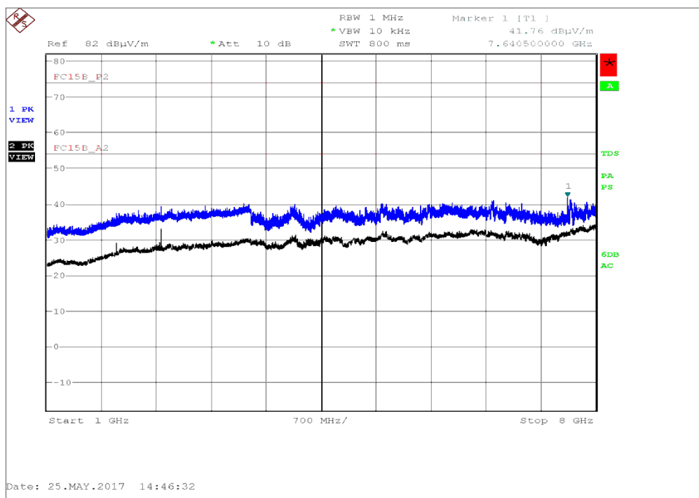
Figure 6 - Graphical Results - 1 GHz to 8 GHz
