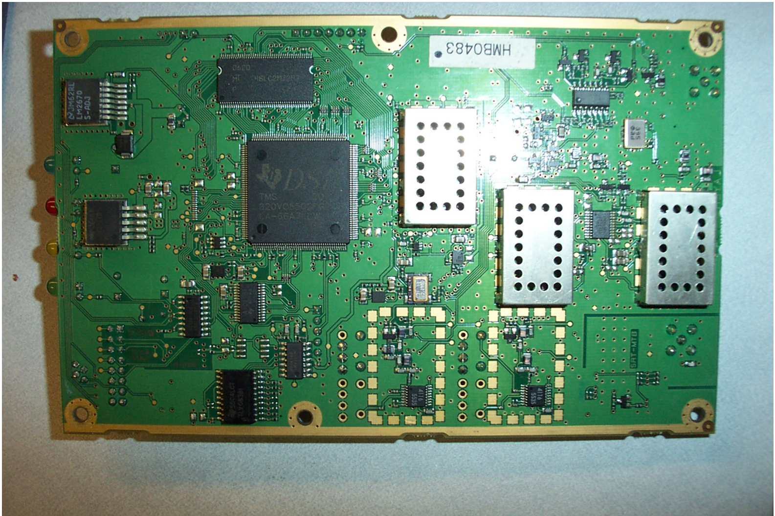
AIS-300 Internal Photos: PCB Bottom
