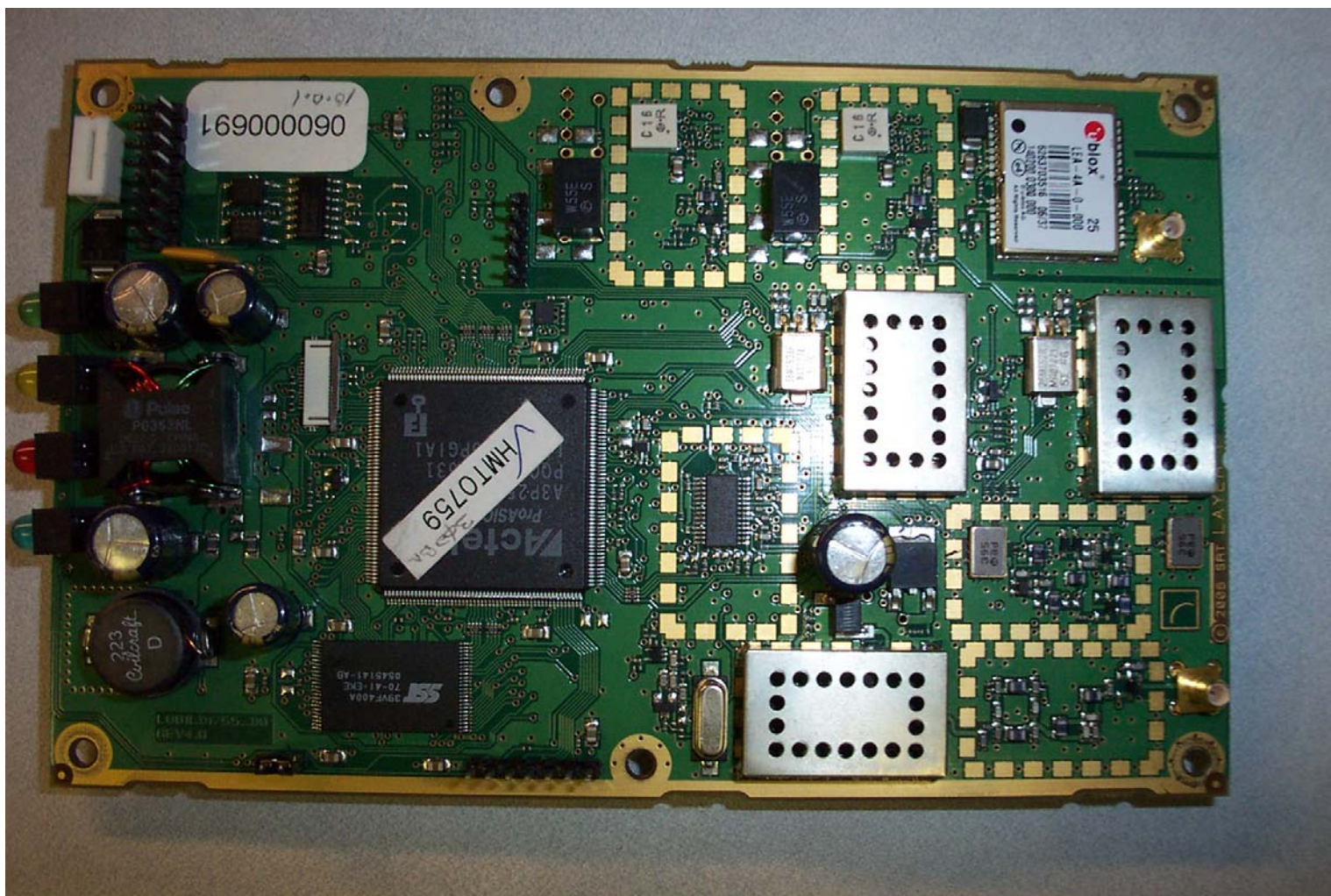
AIS-300 Internal Photos: PCB Top
