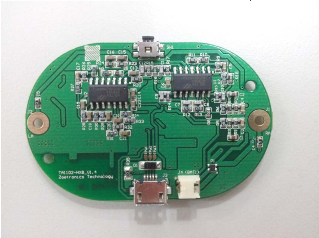
Photo 6 Internal View (Main Board, Back View)
