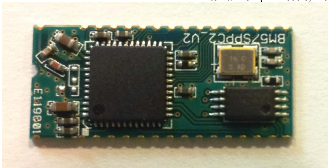
Photo 7 Internal View (BT Module, Front View)
