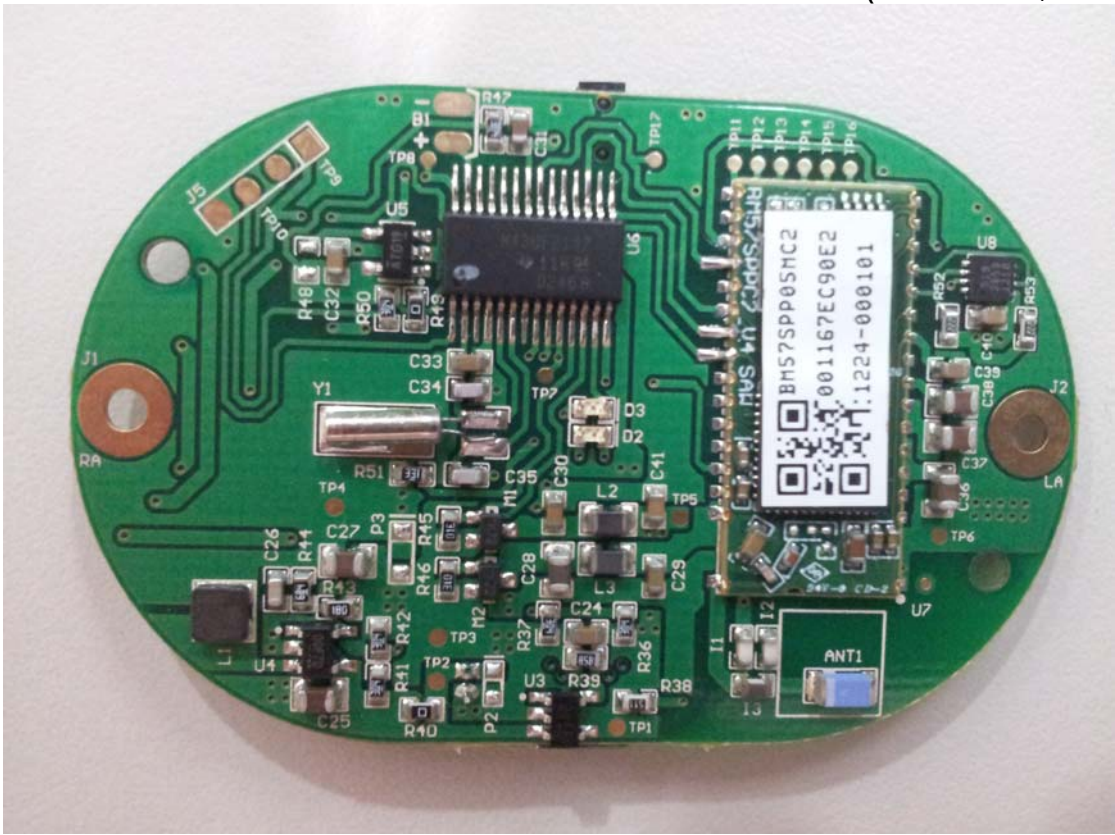
Photo 5 Internal View (Main Board, Front View)
