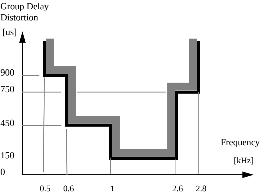
Figure 8. Group delay distortion with frequency
