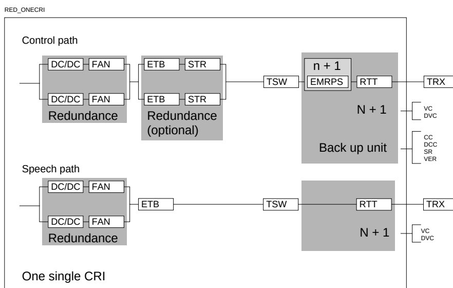
Figure 14 One CRI, system structure, logically
