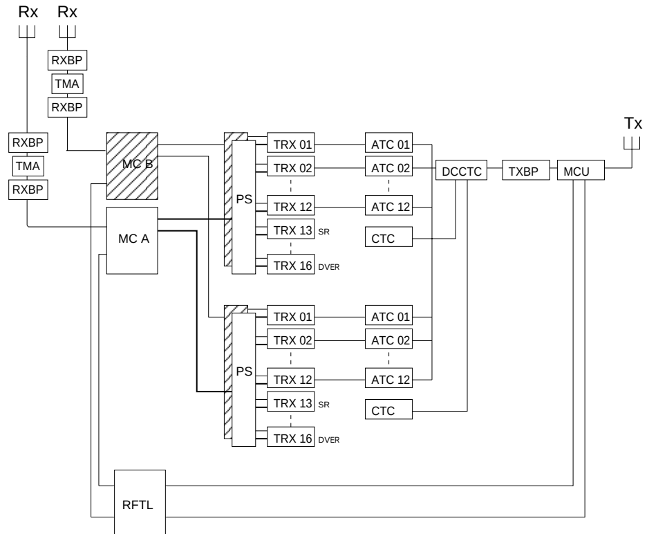
Figure 11 The RF structure including TMA.
