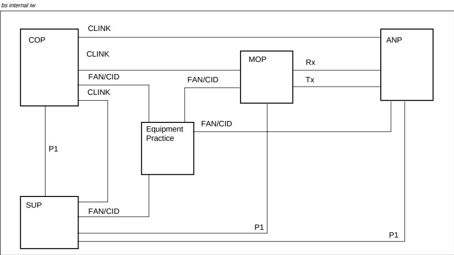
Figure 7 RBS884 Internal Interfaces, physical level.
