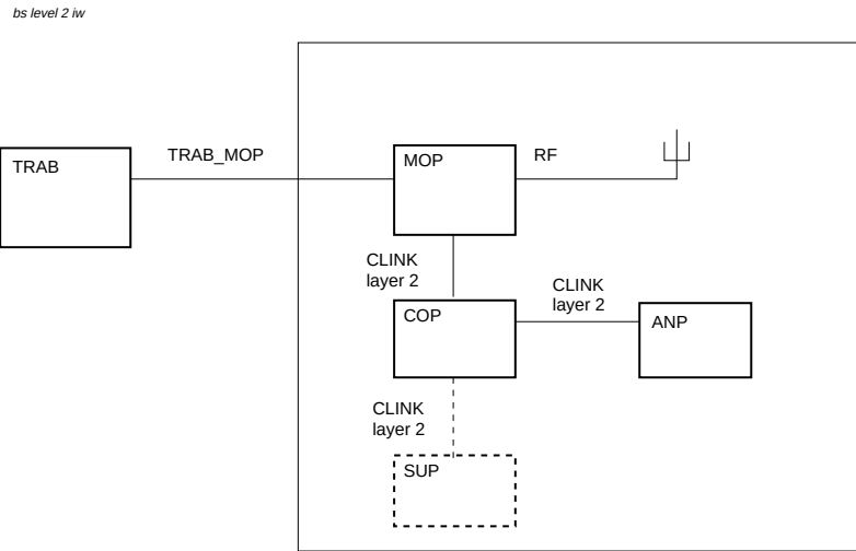
Figure 8 RBS884 Internal Interfaces, level 2. Dotted lines shows future interwork.
