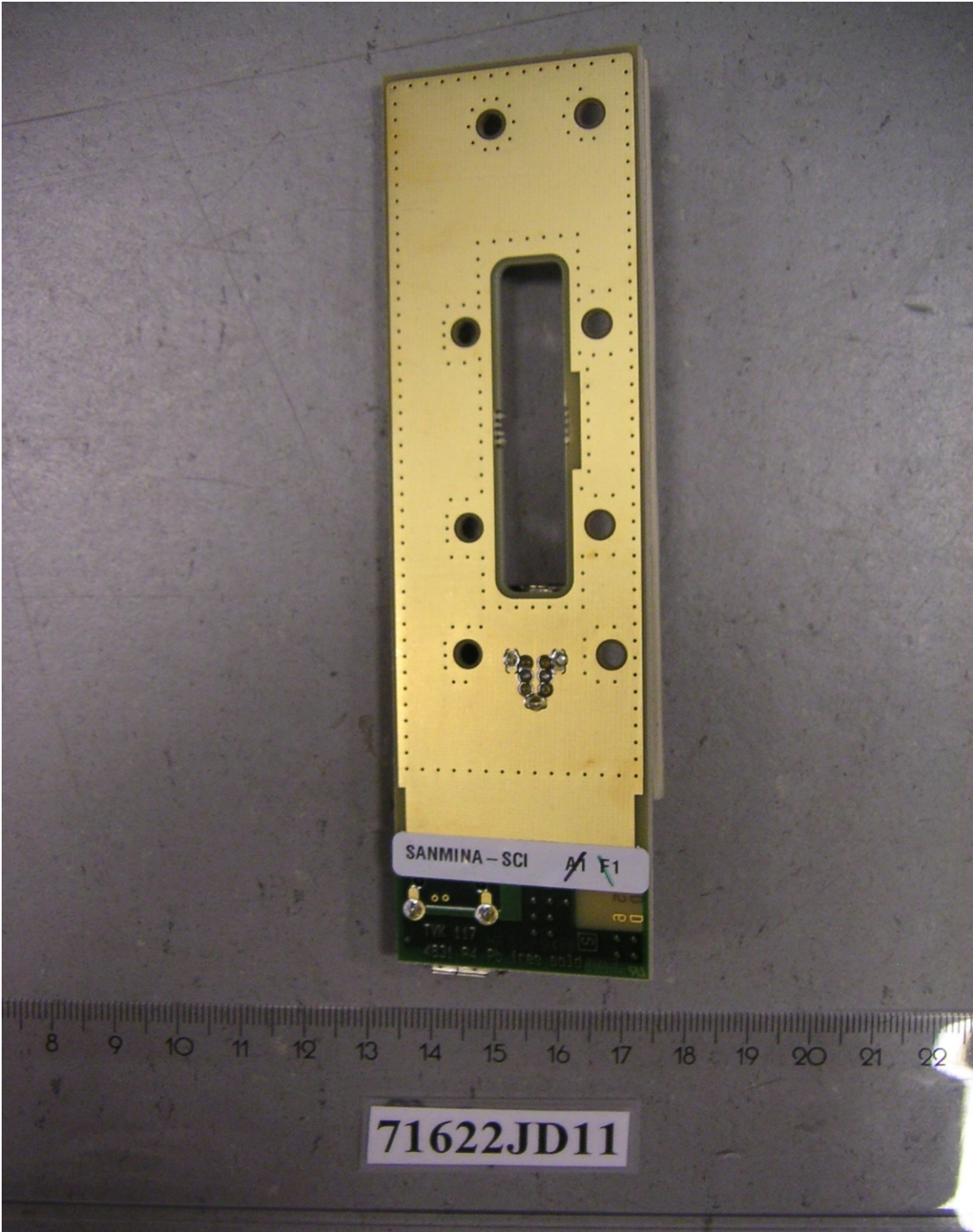
PHT/71622JD11/027 Y Interface Board. Back View
