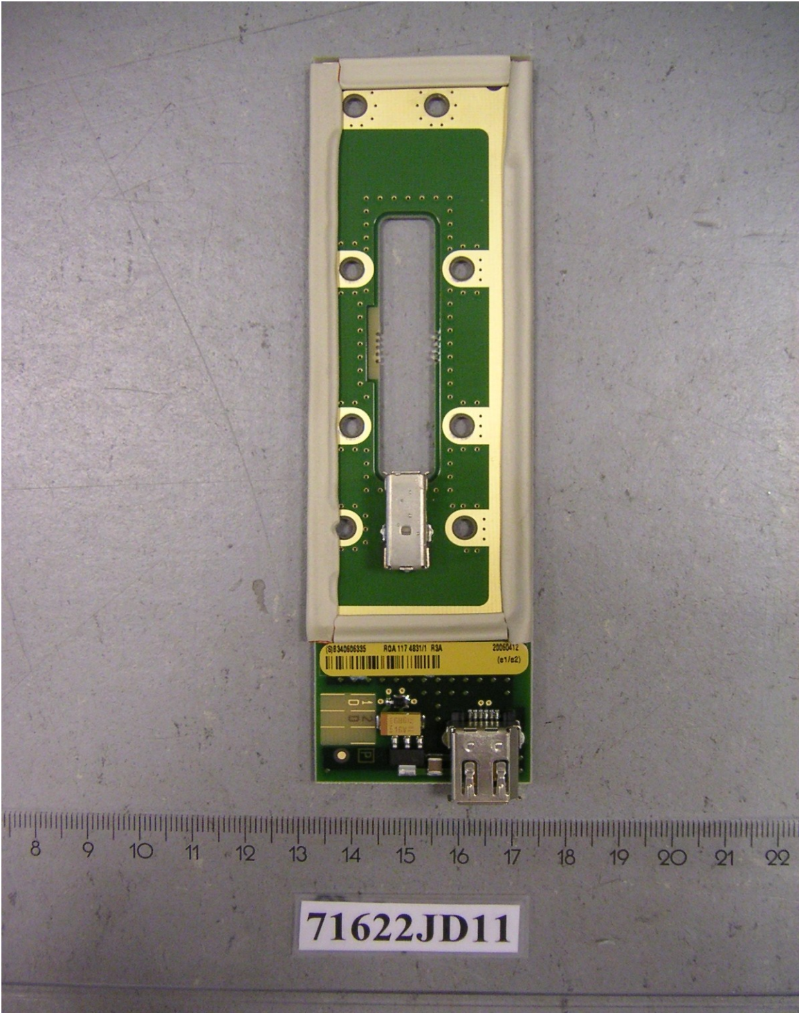
PHT/71622JD11/026 Y Interface Board. Front View
