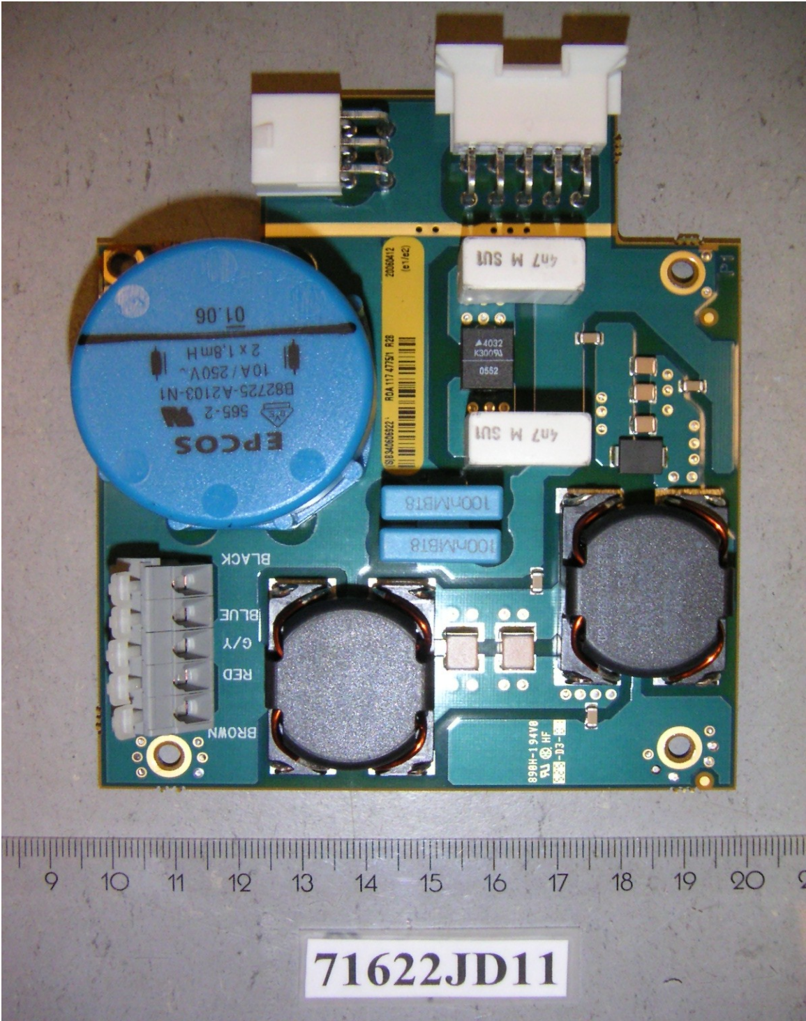
PHT/71622JD11/028 Power Interface Board. Front View
