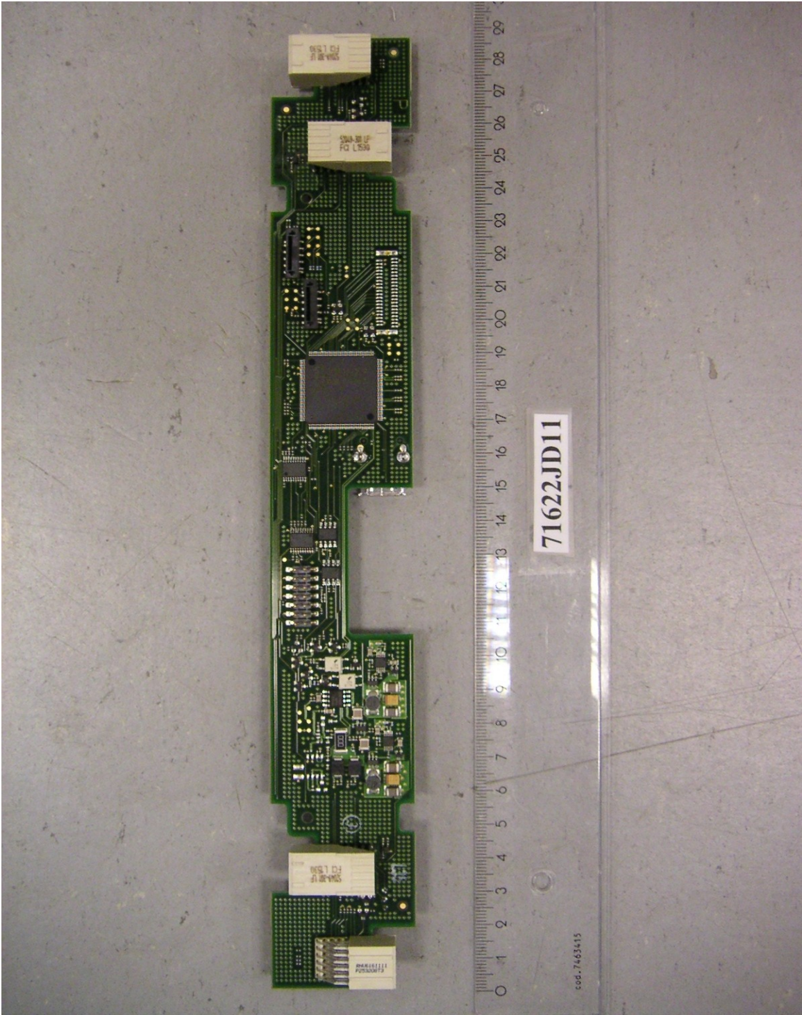
PHT/71622JD11/025 Radio Interface Board. Back View
