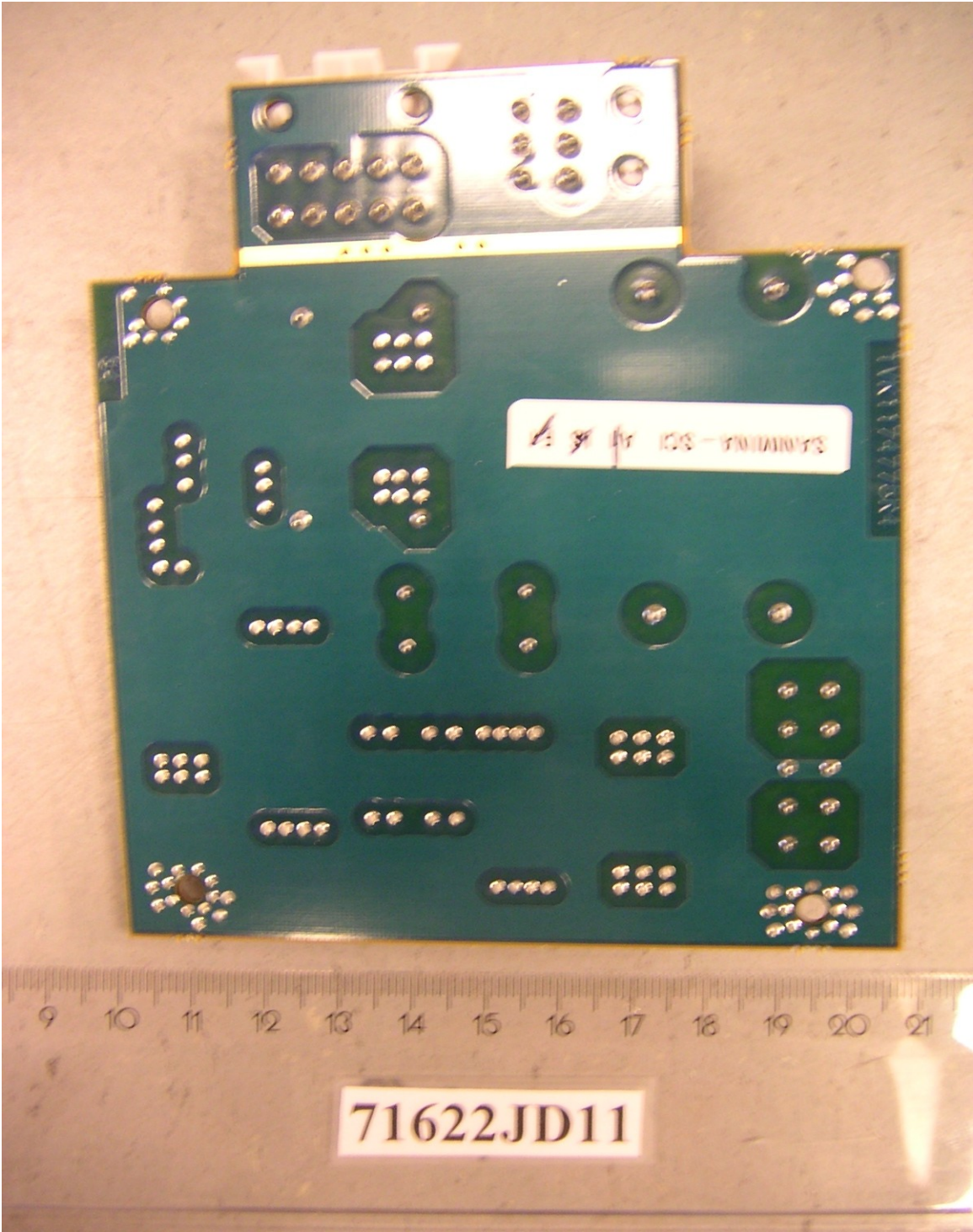
PHT/71622JD11/029 Power Interface Board. Back View
