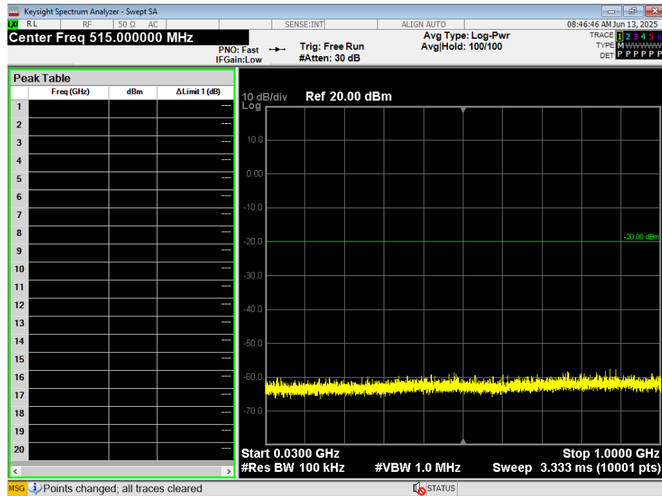
Figure 7 - Conducted Spurious Plot, GMSK 1MB, 30MHz – 1GHz, High
