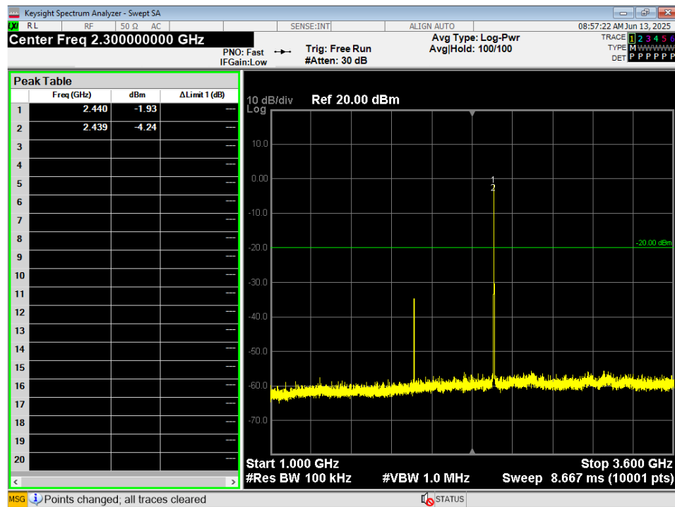
Figure 11 - Conducted Spurious Plot, GMSK 2MB, 1GHz – 3.6GHz, Mid
