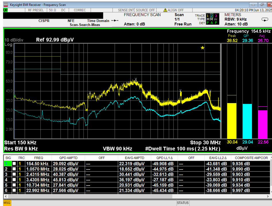
Figure 13 – Conducted Emissions Plot, AC Mains, IDLE, Line
