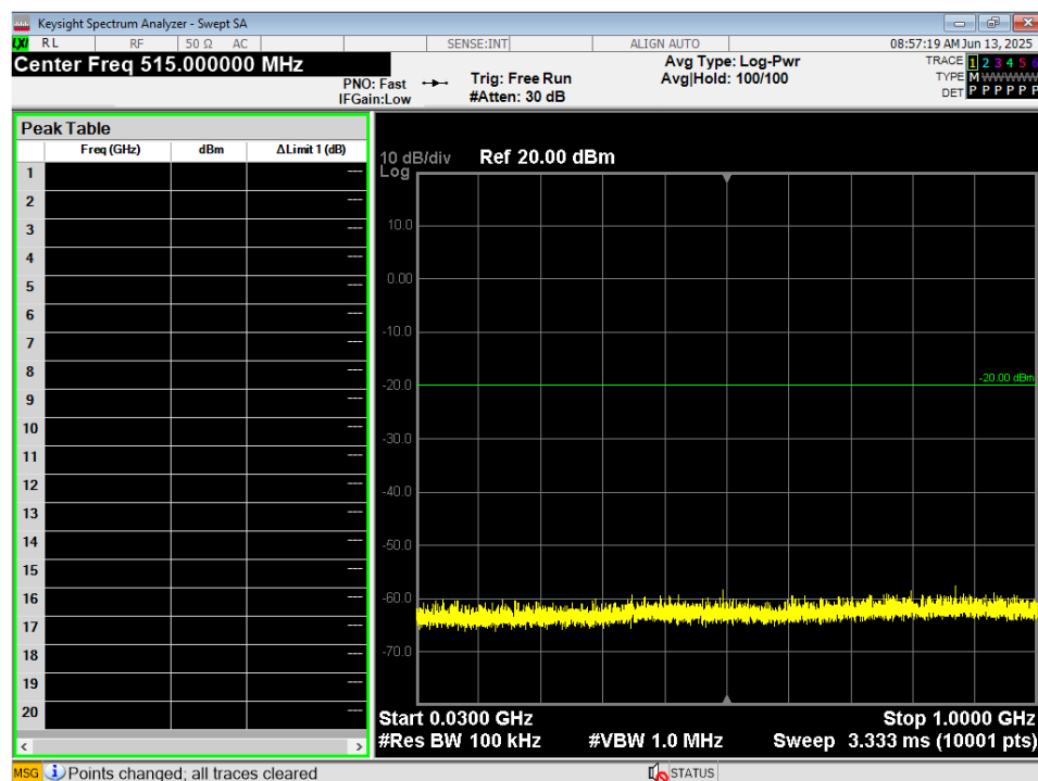
Figure 10 - Conducted Spurious Plot, GMSK 2MB, 30MHz – 1GHz, Mid
