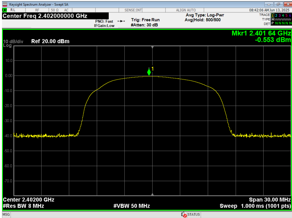
11 Peak Power, BLE 1MB, 2402MHz
