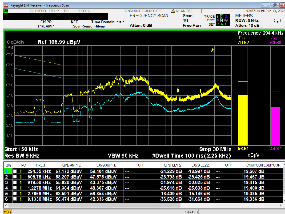
Figure 18 – Conducted Emissions Plot, Telecom, Right Port
