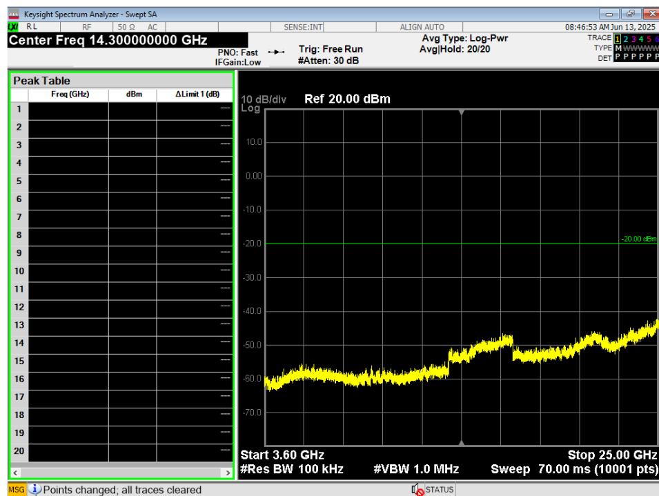
Figure 9 - Conducted Spurious Plot, GMSK 1MB, 3.6GHz – 25GHz, High
