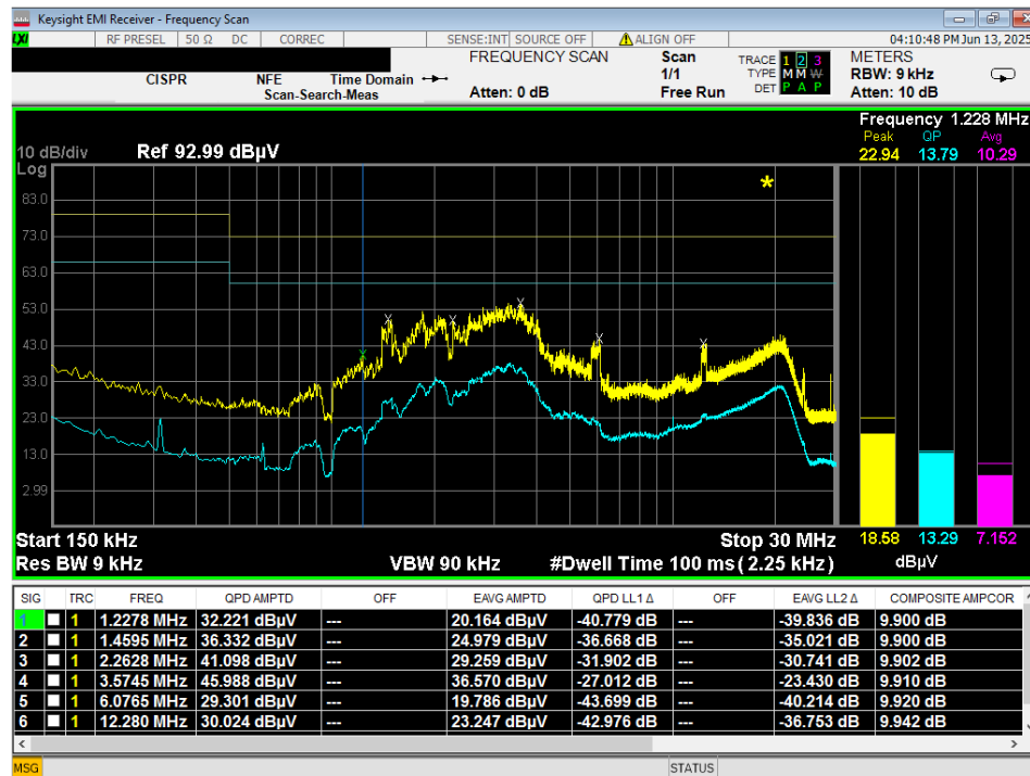
Figure 16 – Conducted Emissions Plot, AC Mains, TX, Neutral
