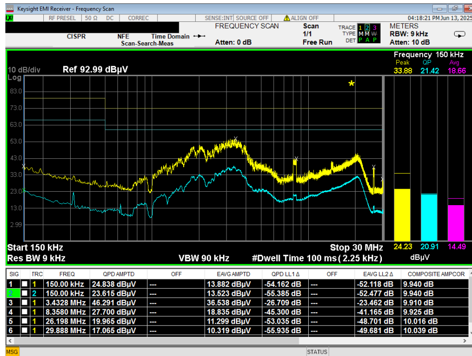
Figure 14 – Conducted Emissions Plot, AC Mains, IDLE, Neutral
