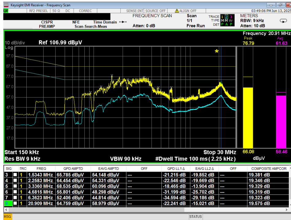
Figure 17 – Conducted Emissions Plot, Telecom, Left Port
