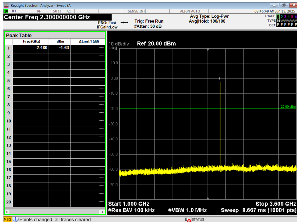
Figure 8 - Conducted Spurious Plot, GMSK 1MB, 1GHz – 3.6GHz, High
