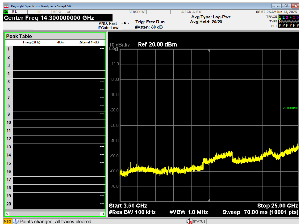
Figure 12 - Conducted Spurious Plot, GMSK 2MB, 3.6GHz – 25GHz, Mid
