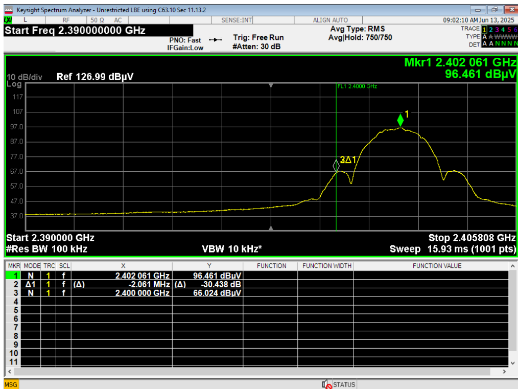
23 LBE Unrestricted AVG, BLE 2MB, 2402MHz
