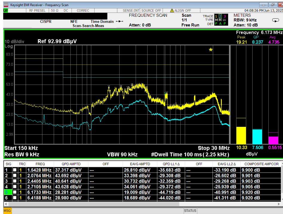
Figure 15 – Conducted Emissions Plot, AC Mains, TX, Line
