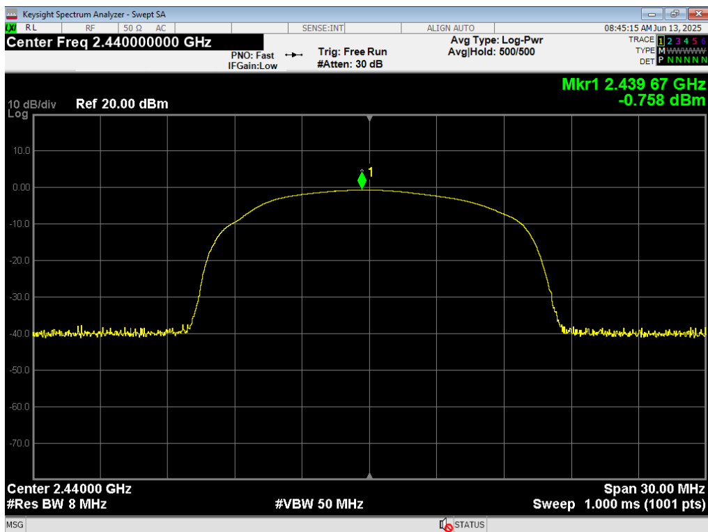
12 Peak Power, BLE 1MB, 2440MHz
