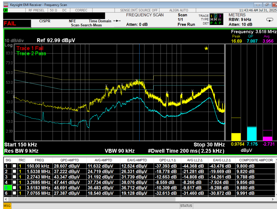
Figure 15 – Conducted Emissions Plot, AC Mains, TX, Line Please disregard failing notification, quasi-peak is below limit line.
