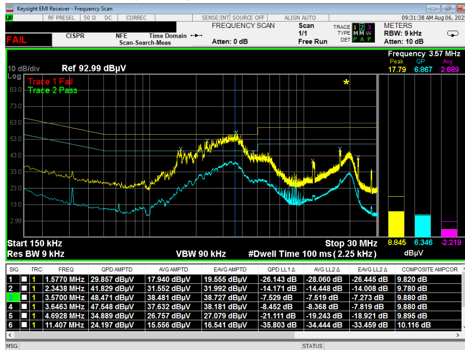
Figure 16 – Conducted Emissions Plot, AC Mains, TX, Neutral Please disregard failing notification, quasi-peak is below limit line.
