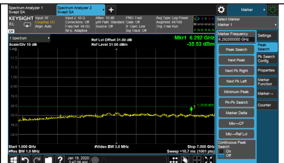
Low Channel - Above 1 GHz
