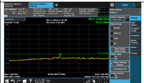
Middle Channel - Above 1 GHz
