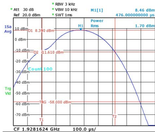
PSD CHAIN 0- Channel 0
