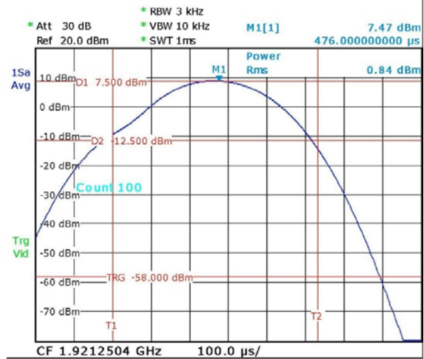
PSD CHAIN 1- Channel 4
