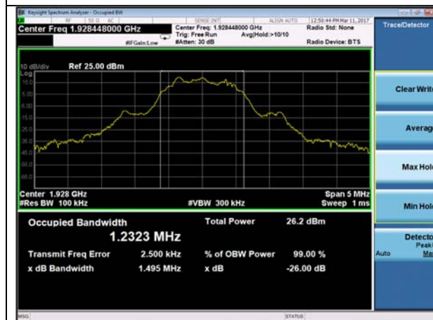
99%OBW -26dB bandwidth-Channel 0
