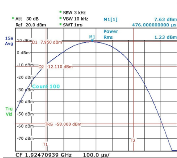
PSD CHAIN 0- Channel 0
