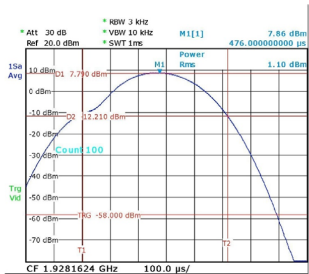
PSD CHAIN 1- Channel 4
