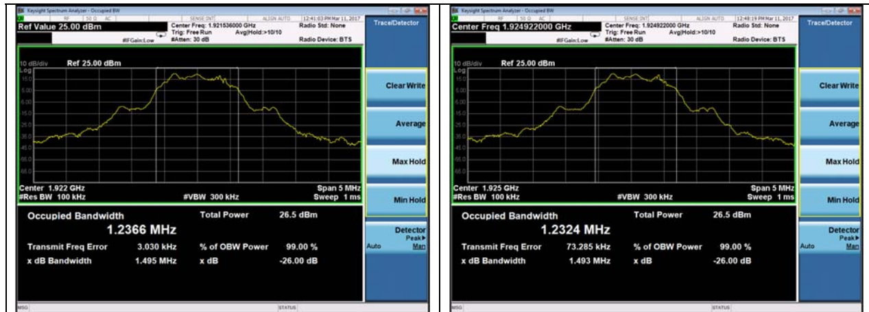
99%OBW -26dB bandwidth-Channel 4
