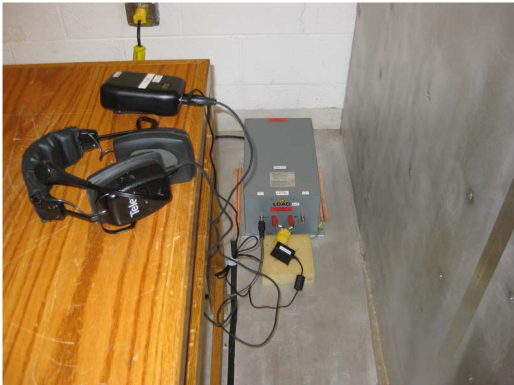
Conducted Emissions #2
