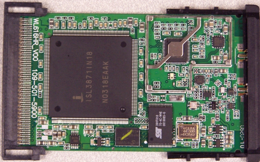
RF Card without Internal Shield - Top View
