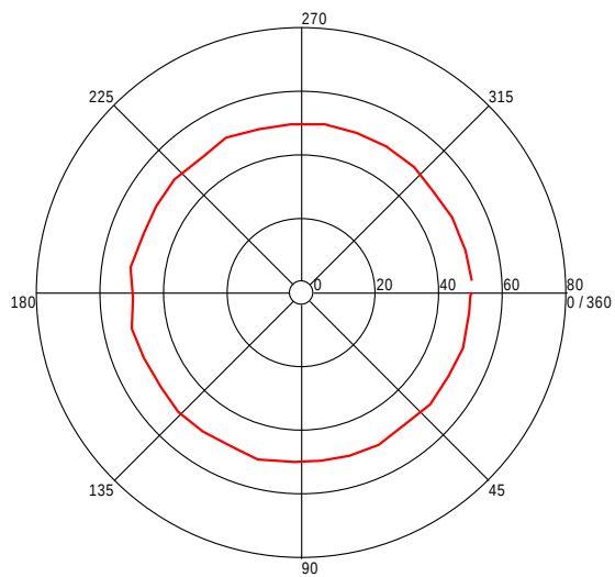
Turntable Plot ( 8.347080829 GHz )
