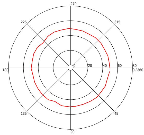
Turntable Plot ( 7.482672011 GHz )
