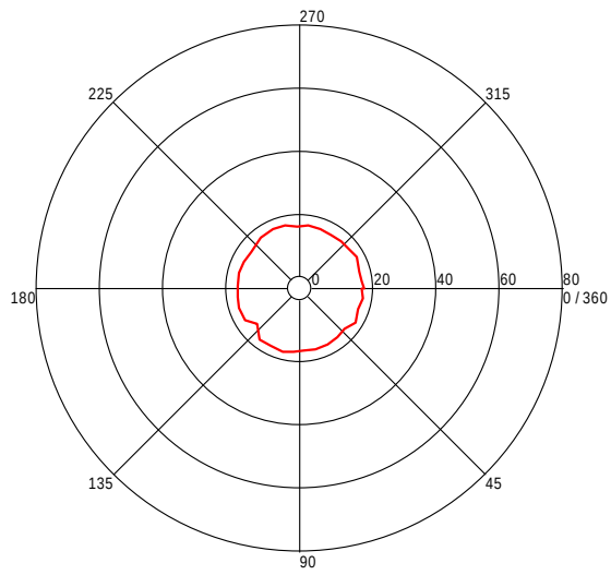
Turntable Plot ( 122.41623207 MHz )
