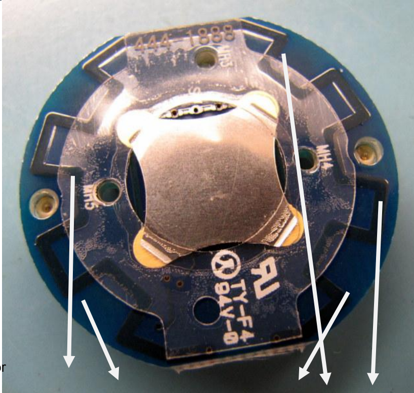
Button Side – Antenna trace surrounds switch
