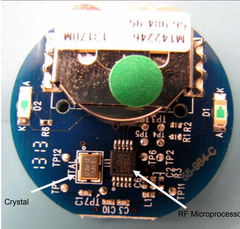
Component Side
