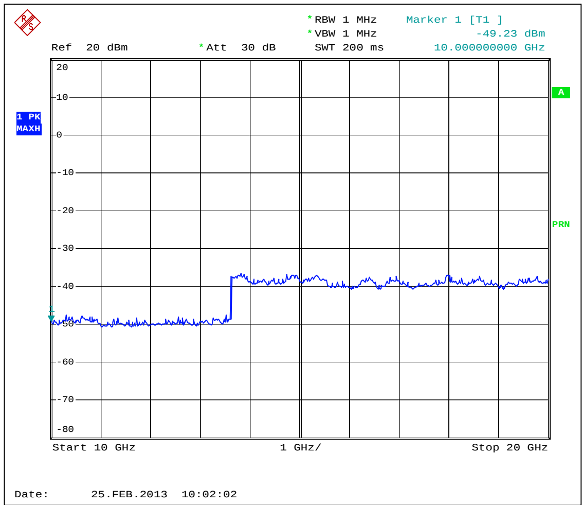
Graph 3.5.3
