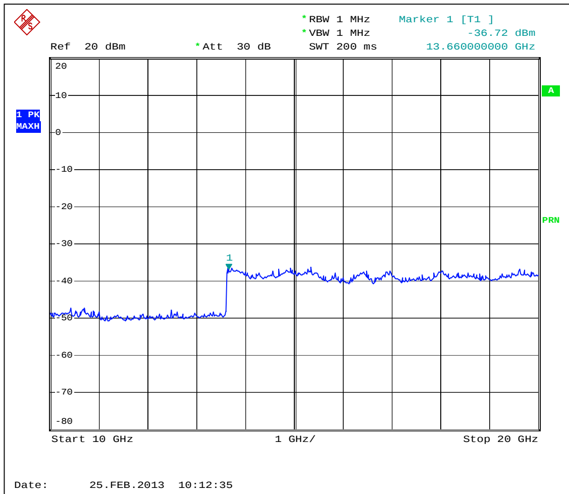
Graph 3.5.9
