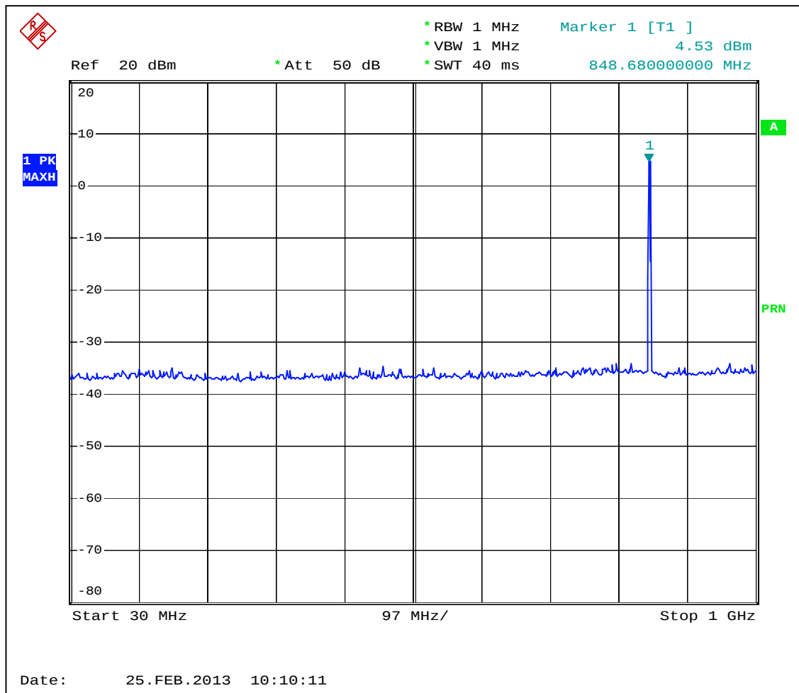
Graph 3.5.7
