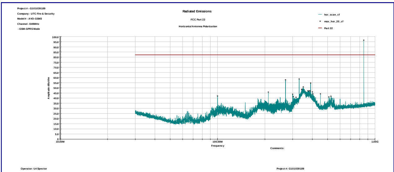
Graph 3.6.9
