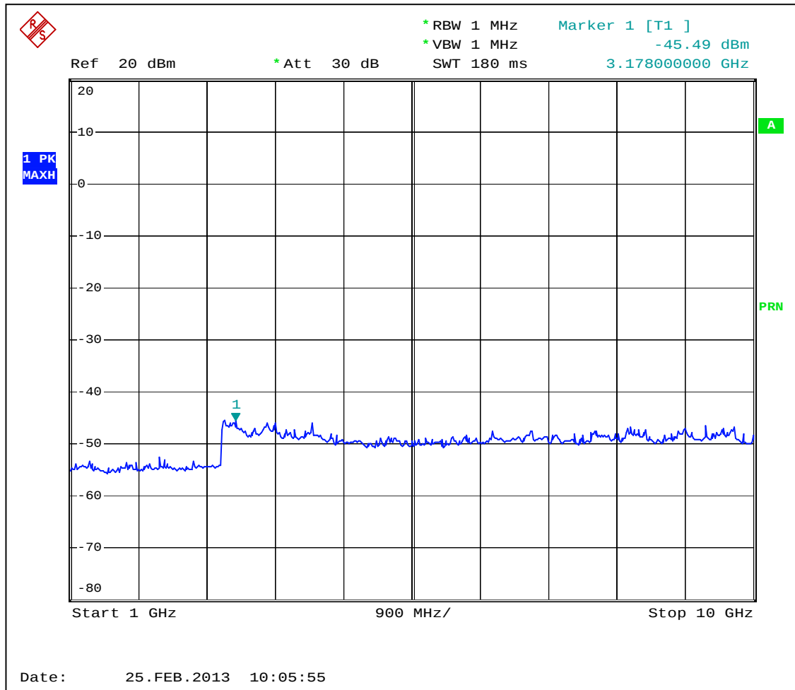
Graph 3.5.5
