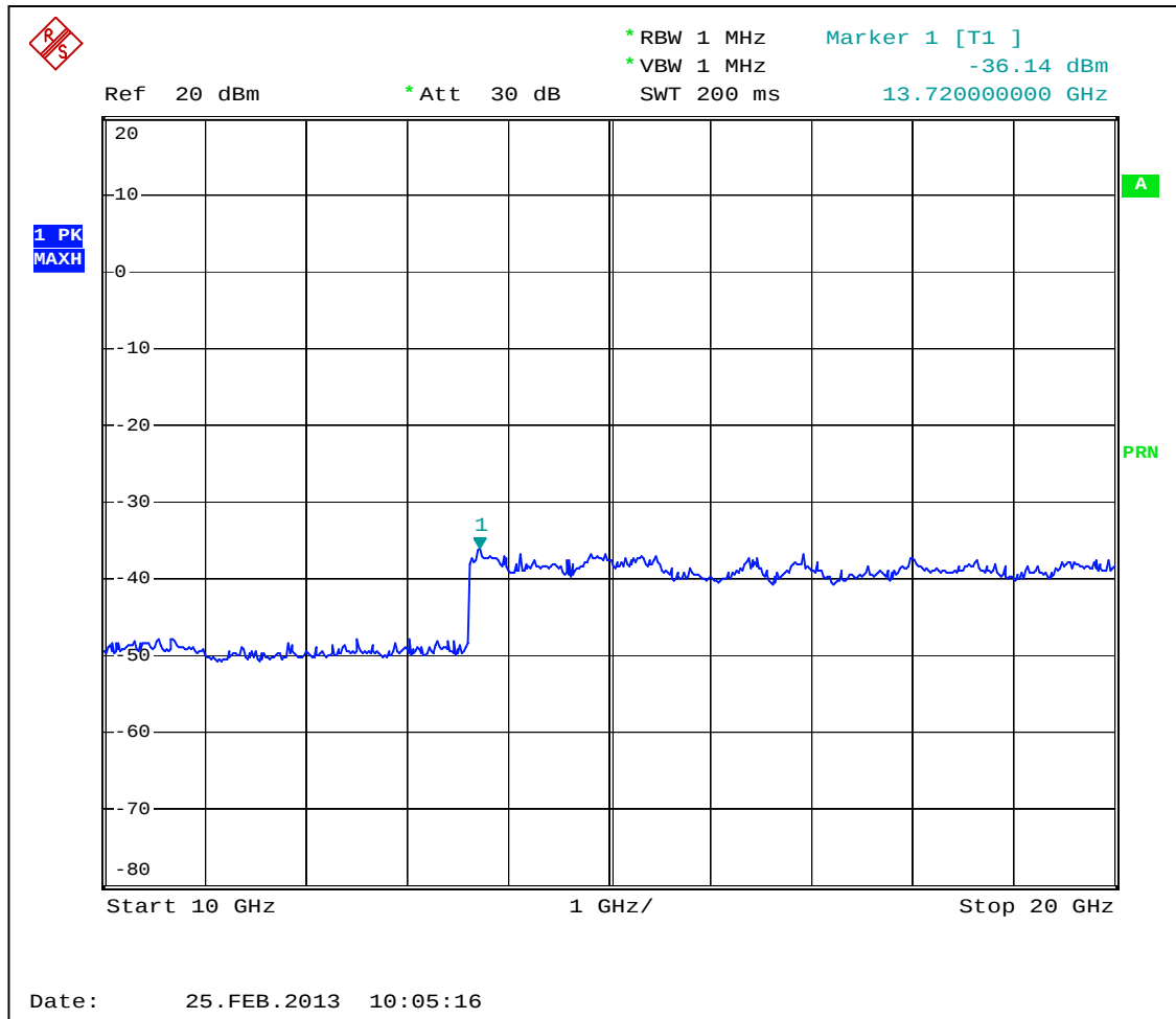
Graph 3.5.6
