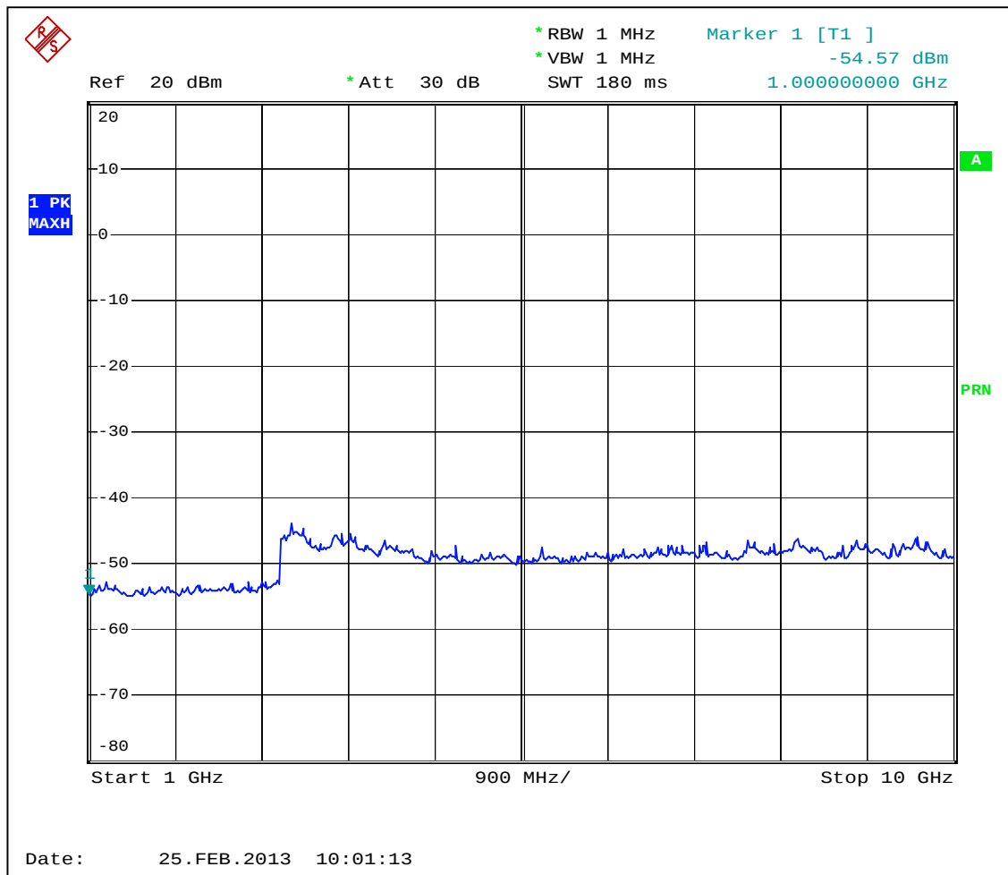
Graph 3.5.2
