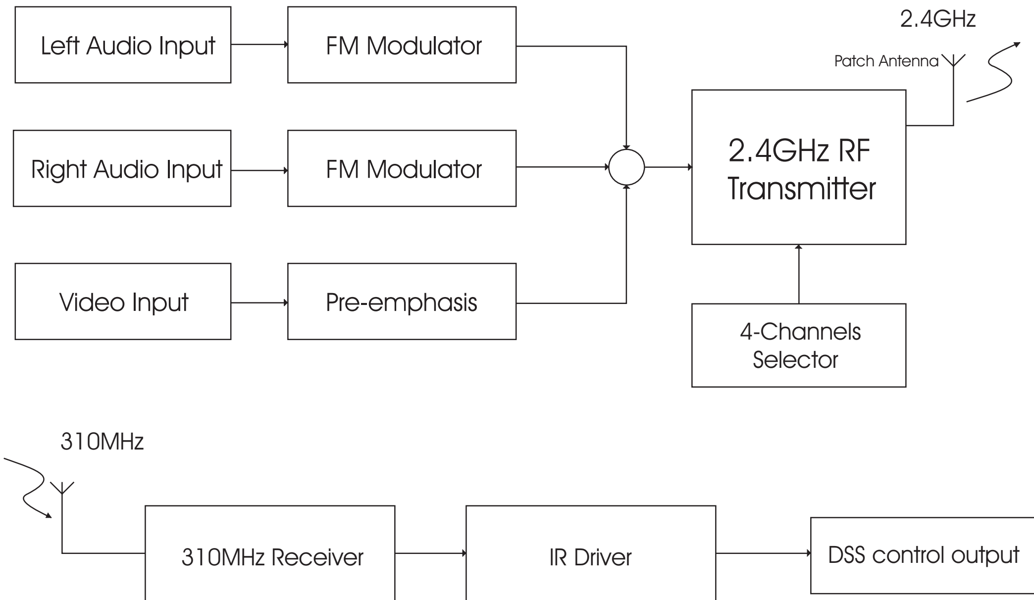
Block Diagram for Video Sender Transmitter (VT30A)
