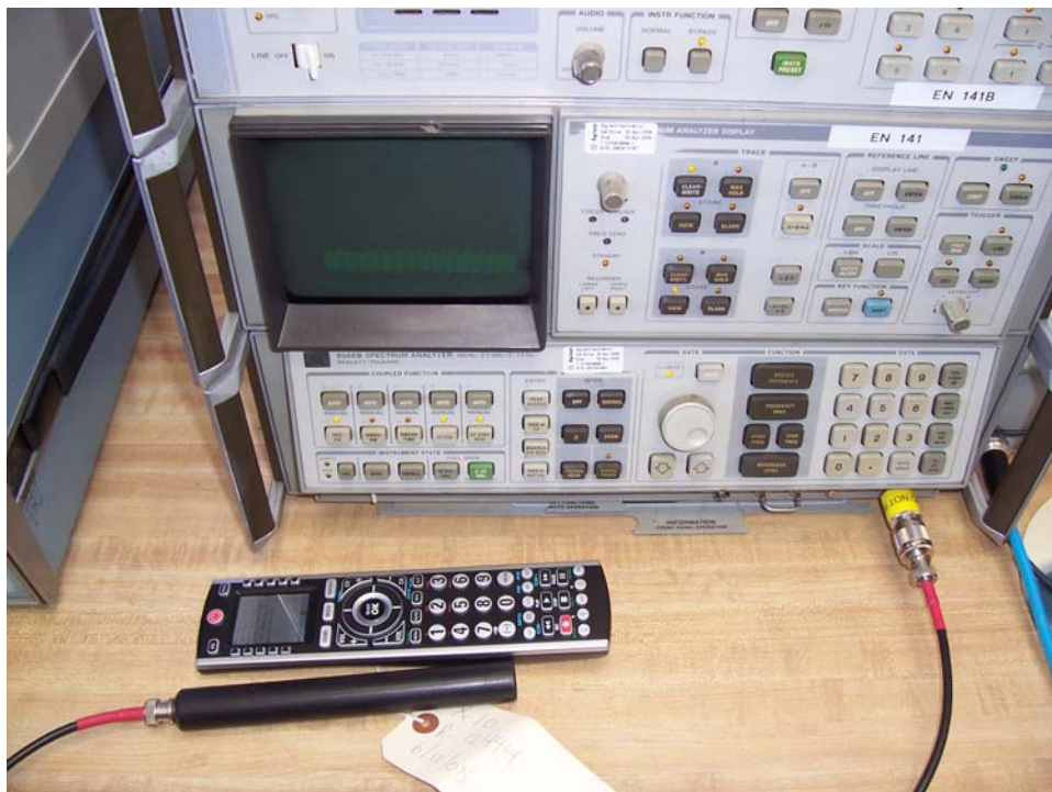
Duty Cycle and Occupied Bandwidth, Test Setup
