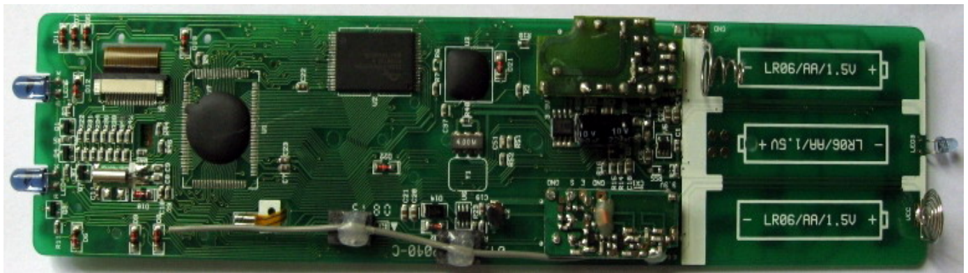
Main PC Board bottom view
