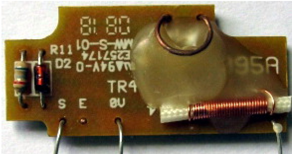
310 MHz PC Board top view
