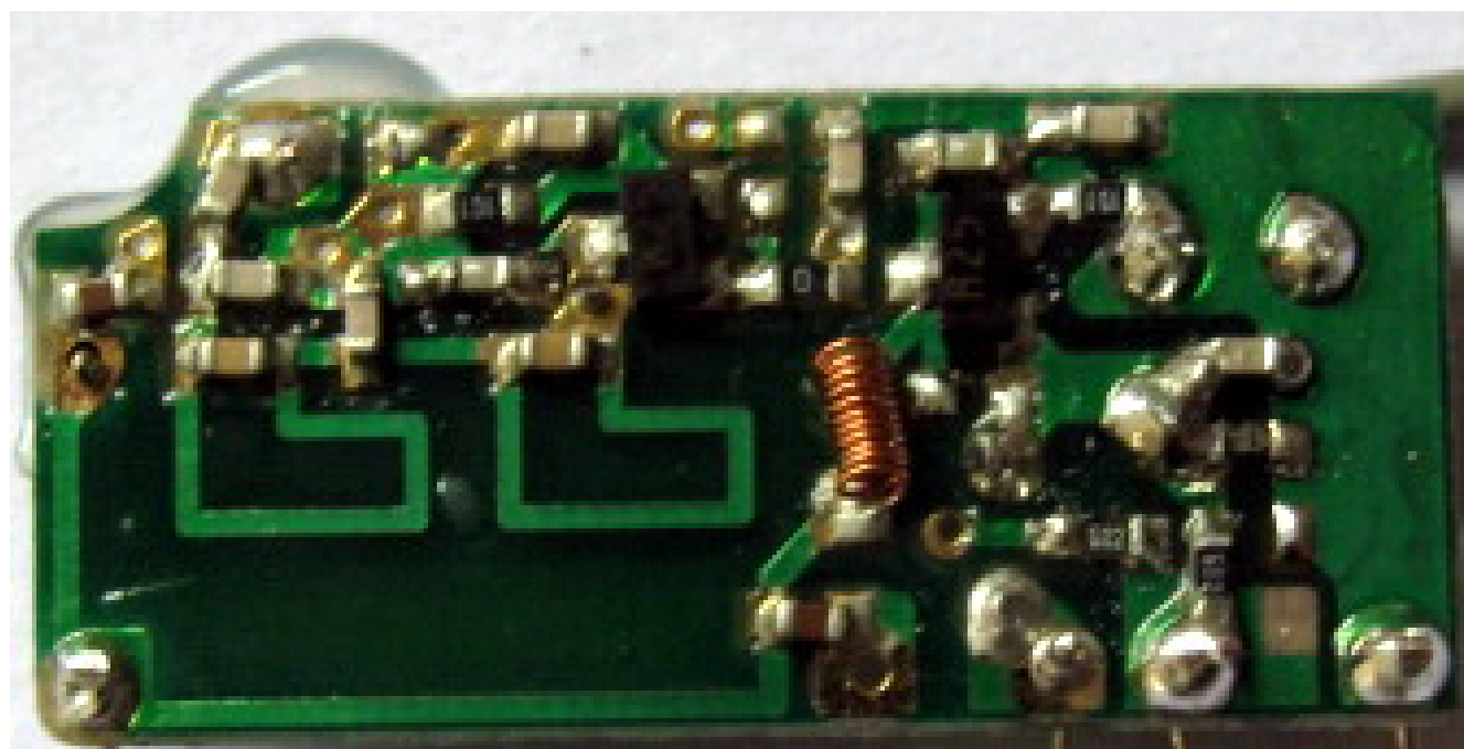
433 MHz PC Board bottom view
