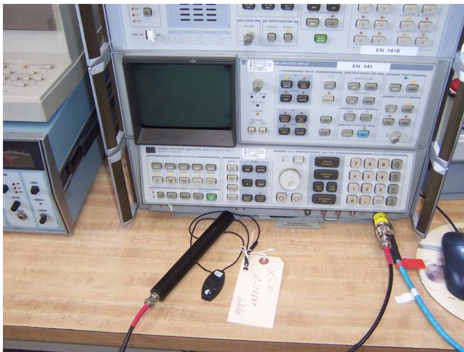
Duty Cycle, Occupied Bandwidth Test Setup
