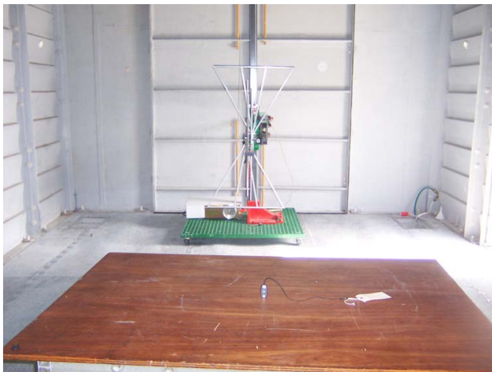
Radiated Emissions, Biconilog Vertical Test Distance Setup
