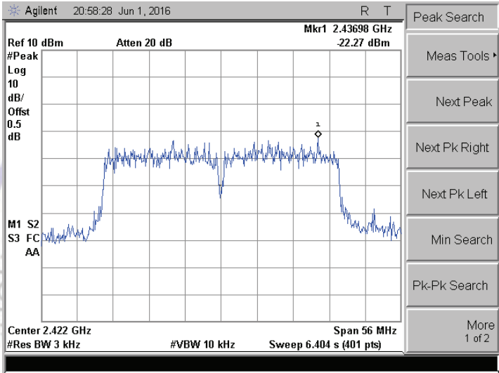
Channel 03 (2422MHz)
