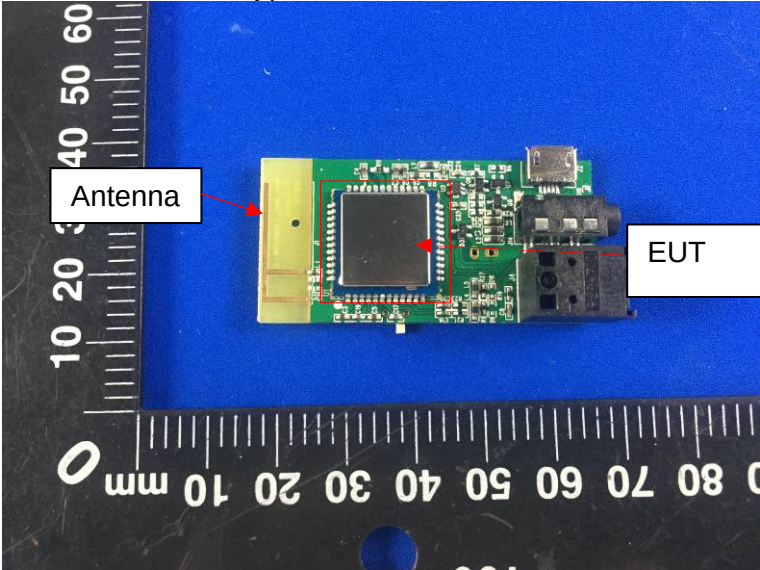
BC870FNA with type 2 antenna: Extend PCB antenna
