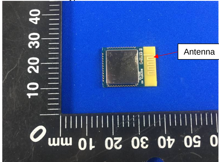
BC870FPA with type 3 antenna: On board PCB antenna
