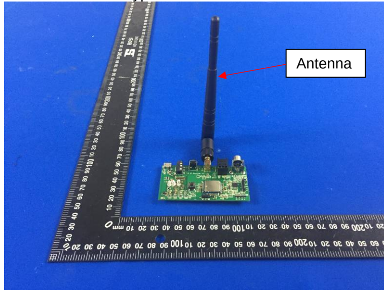
BC870FNA with type 1 antenna: External rod antenna
