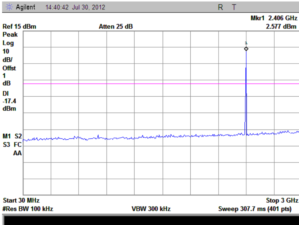
(Plot D.1: Channel = 0, 30MHz to 3GHz @ \pi/4 -DQPSK)
