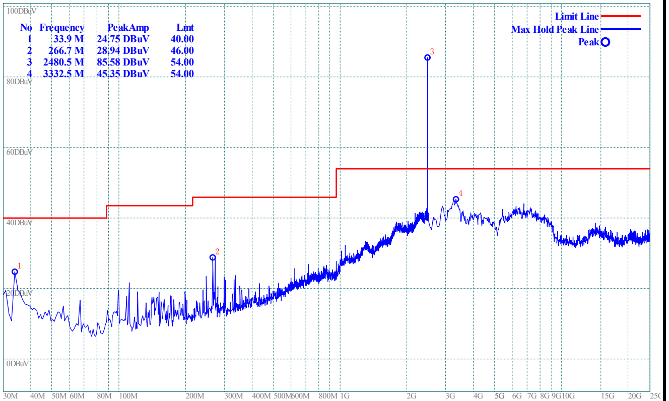
(Plot C.2: 30MHz to 25GHz, Antenna Vertical @ 8-DPSK, channel 78)
