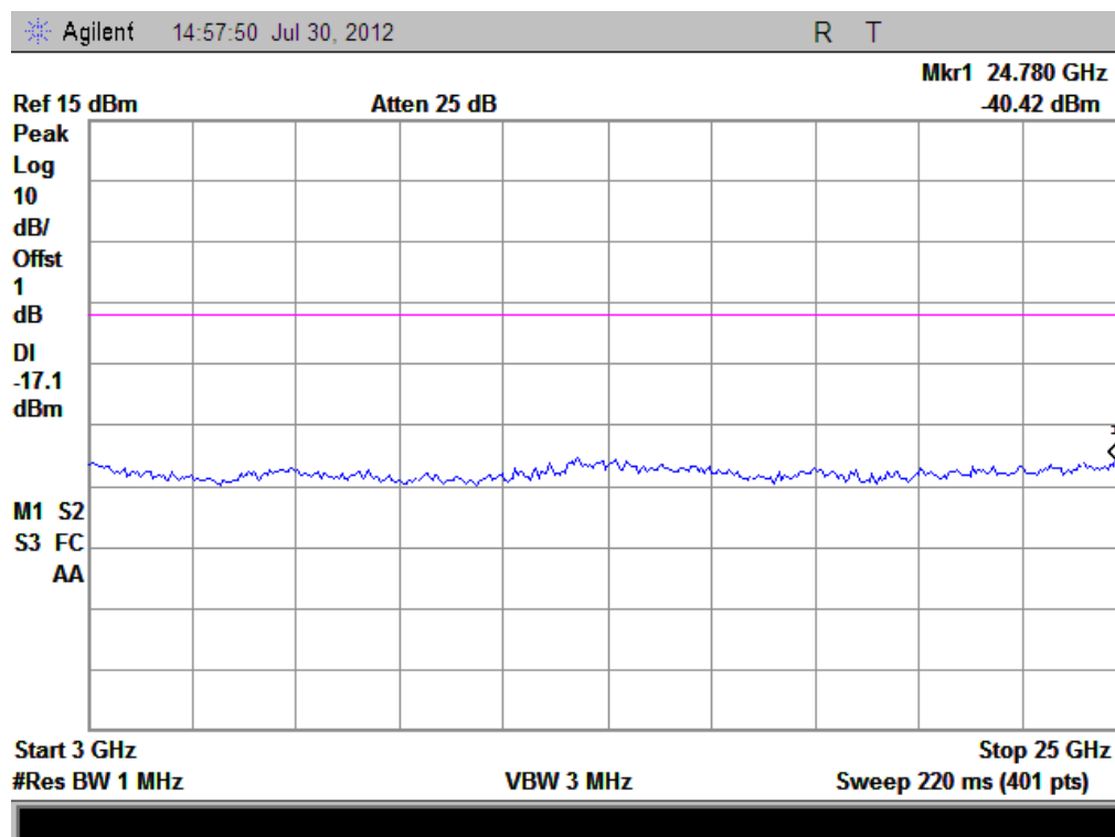
(Plot F.2: Channel = 78, 3GHz to 25GHz @ \pi/4 -DQPSK)
