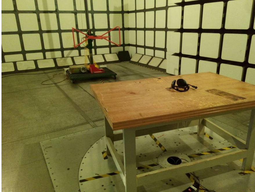
Radiated Emissions View (Below 1 GHz, Single Speaker)
