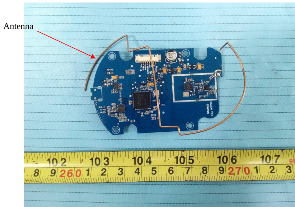
EUT – Mainboard 1 Top Shielding off View
