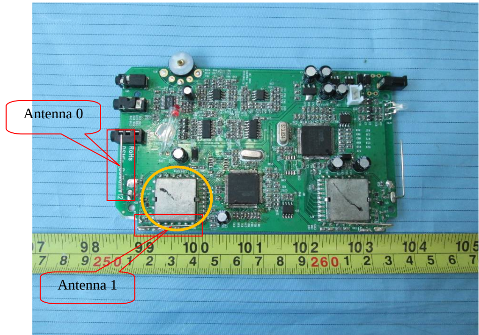
EUT – Testing Jig Board View
