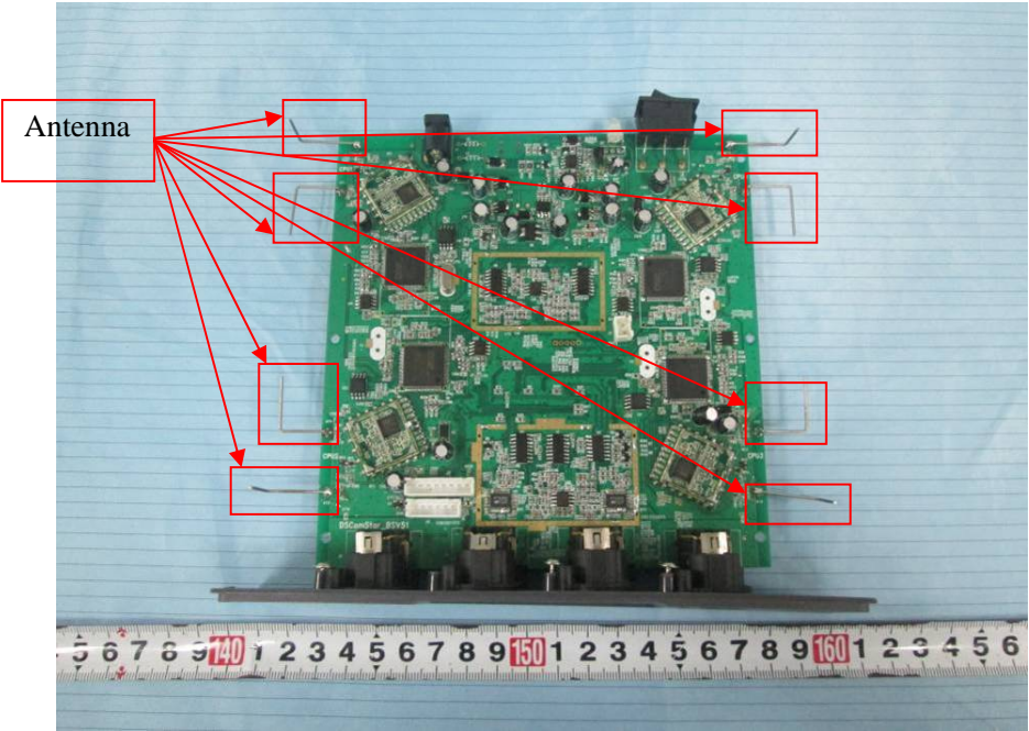
EUT – Main Board 2 Top Shielding off View
