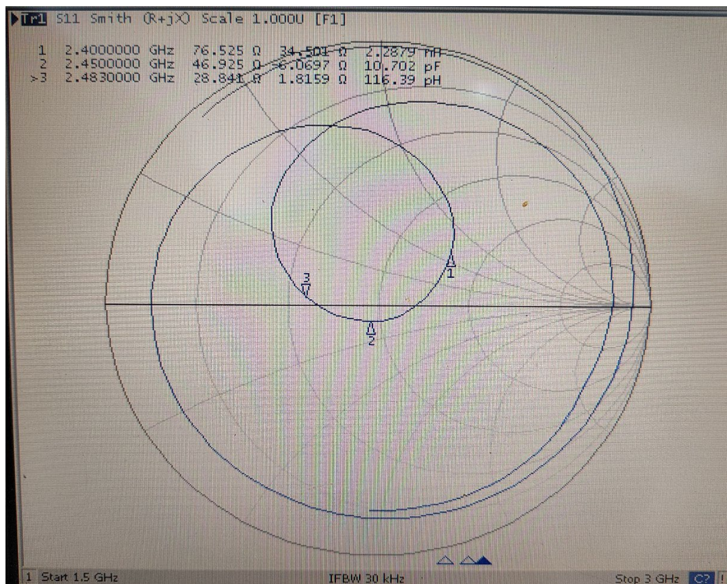
Measured Input Impedance on a Smith Chart
