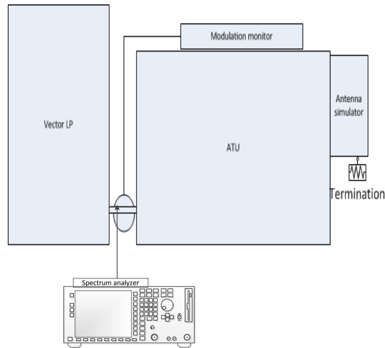
Figure 3.6-1: Setup diagram
