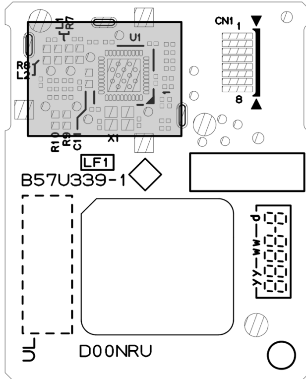
Component Side View
