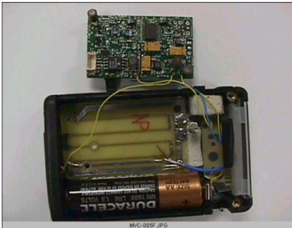
AID2 - FM Transmitter out of Case showing connections, Audio and Microprocessor PCB side and Antenna Board.
