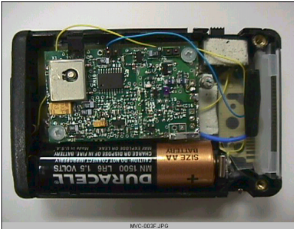
AID2 - PCB Component Side within case showing RF side
