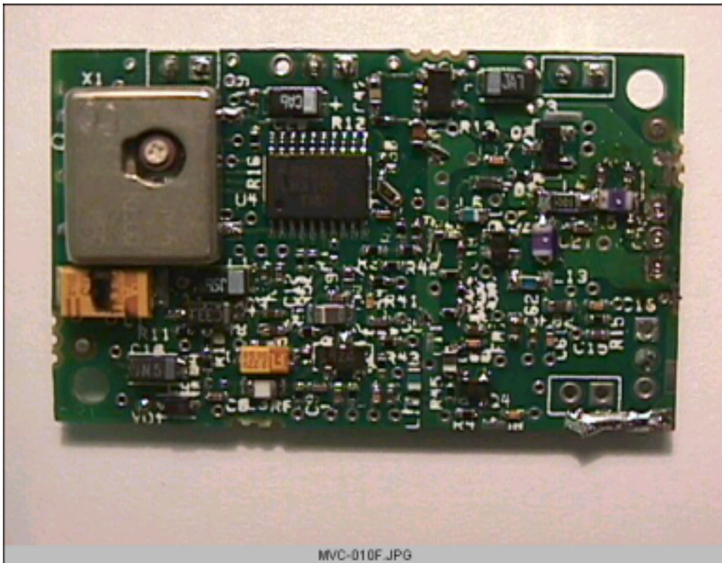
AID2 - PCB showing RF section
