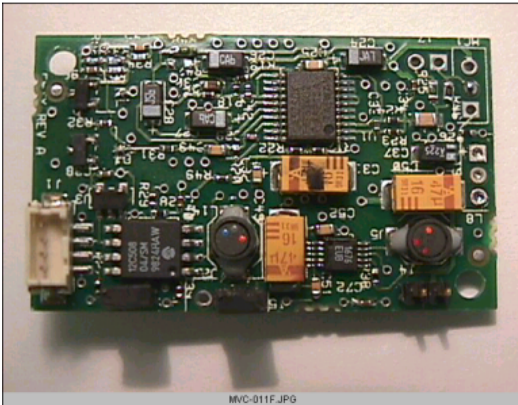
AID2 - PCB showing Audio and Microprocessor side
