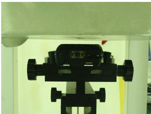
Rear Face of the DUT with Phantom 1 cm Gap
