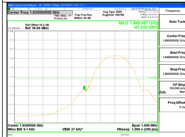
GSM1900 EGPRS Low Channel
