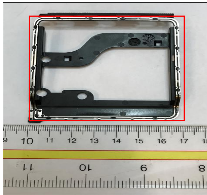
CTLS Antenna
