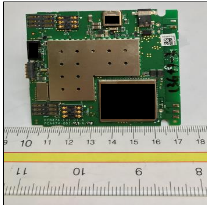
PCB - Top View
