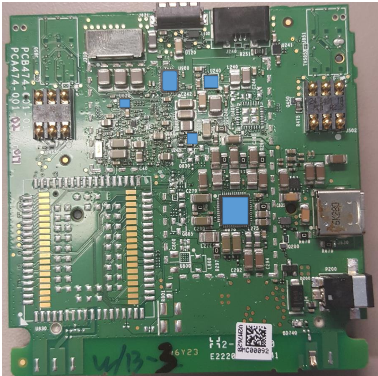
Main Board Back – without shield
