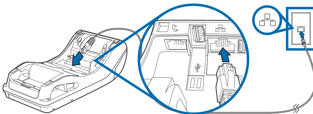
Figure 10 Ethernet Connection
