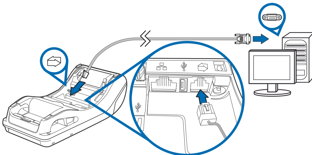
Figure 13 Sample PC Connection
