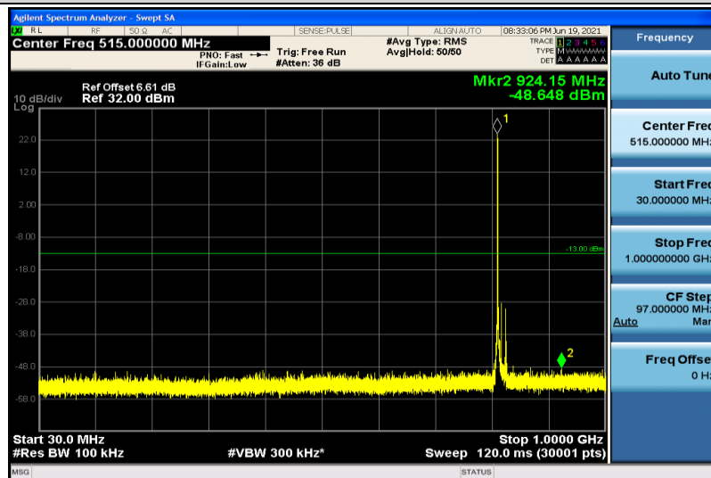
Band26-15MHz-16QAM-26765-1RB#0-30~1000MHz
