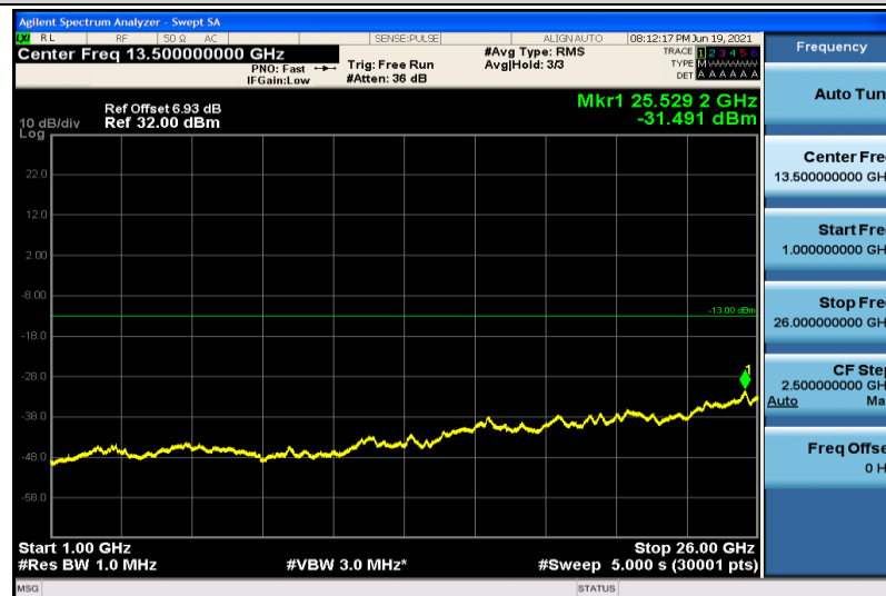
Band26-5MHz-QPSK-26740-1RB#0-1000~26000MHz
