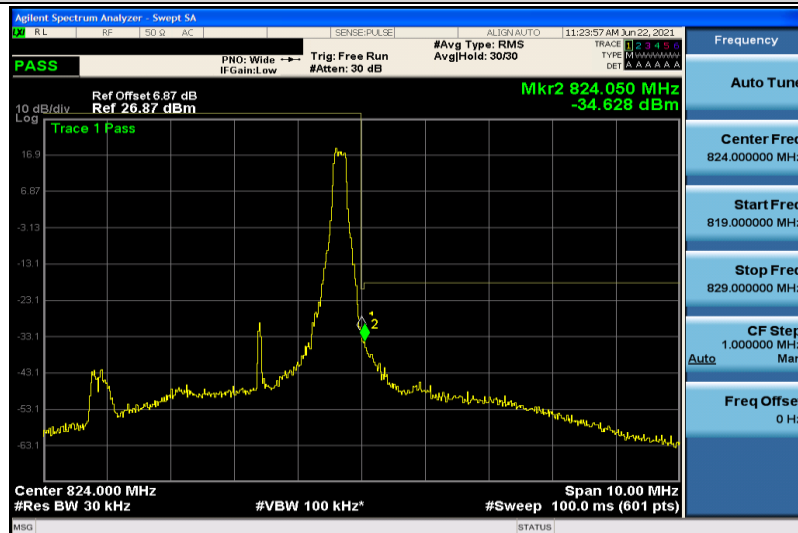
Band26-3MHz-QPSK-26775-1RB#14
