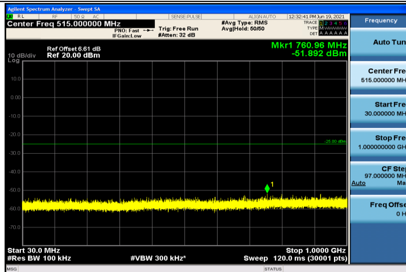
Band7-15MHz-16QAM-21100-1RB#0-30~1000MHz
