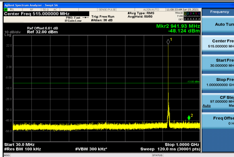
Band5-5MHz-QPSK-20525-1RB#0-30~1000MHz
