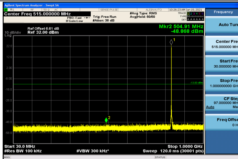
Band5-1.4MHz-16QAM-20525-1RB#0-30~1000MHz
