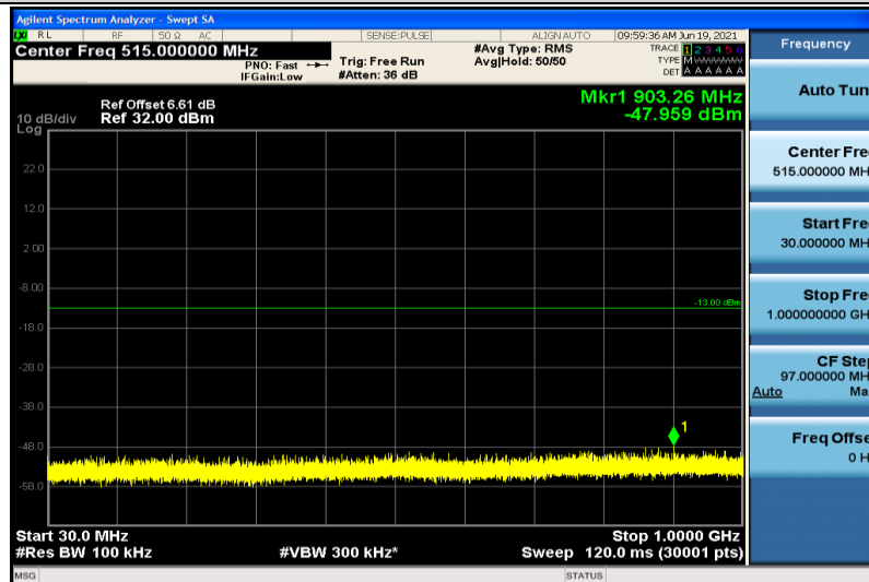
Band4-20MHz-QPSK-20175-1RB#0-30~1000MHz
