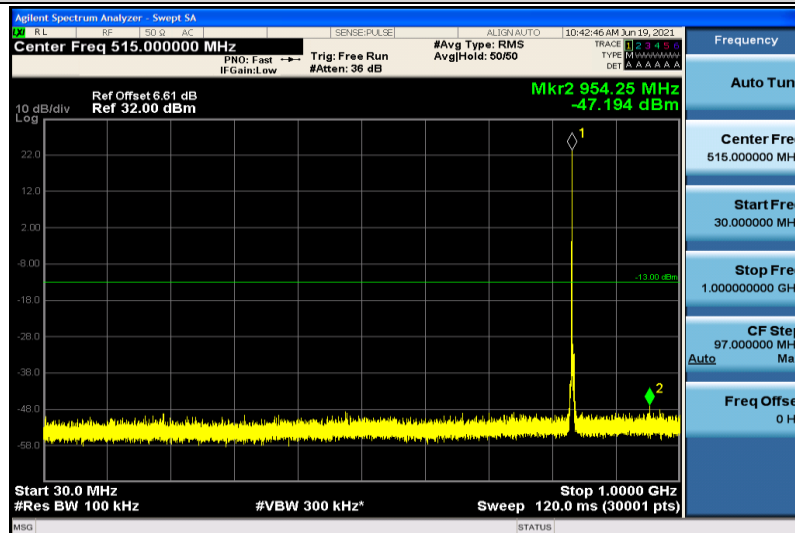
Band5-3MHz-16QAM-20525-1RB#0-30~1000MHz
