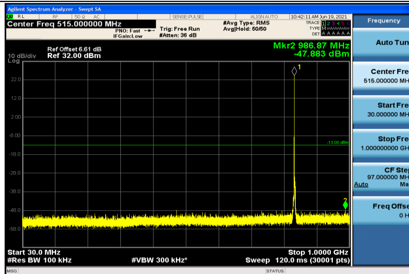
Band5-3MHz-QPSK-20525-1RB#0-30~1000MHz
