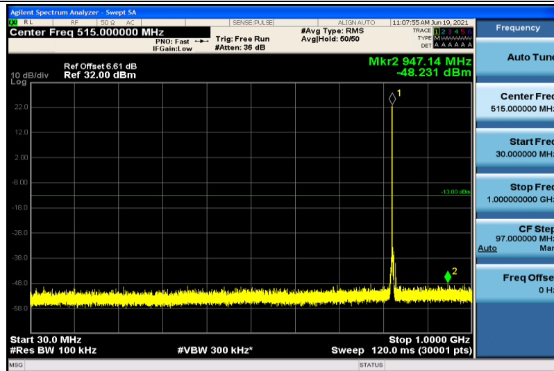
Band5-5MHz-16QAM-20425-1RB#0-30~1000MHz
