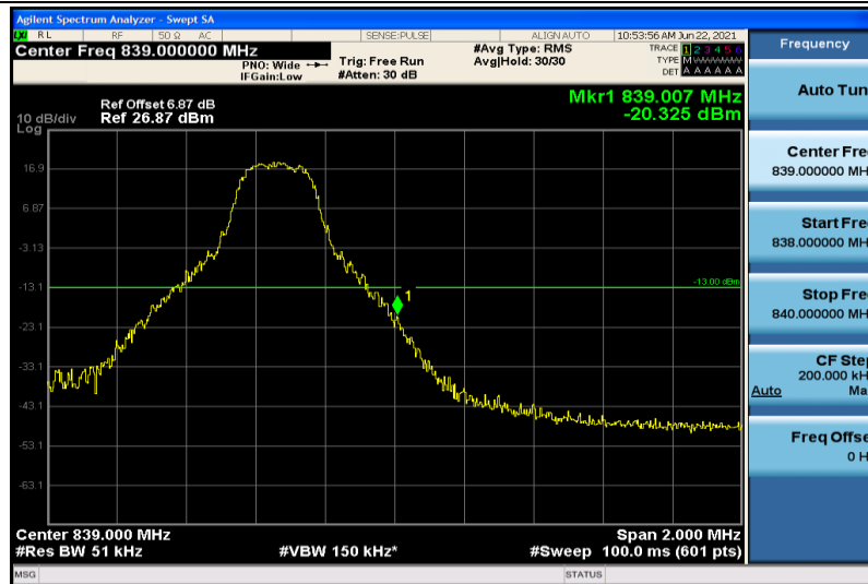
Band26-5MHz-16QAM-26915-1RB#24
