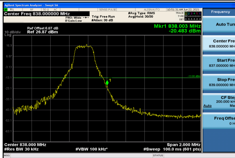
Band26-3MHz-16QAM-26915-1RB#14
