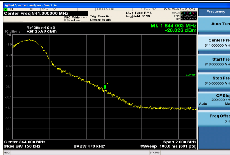
Band26-15MHz-16QAM-26915-1RB#74
