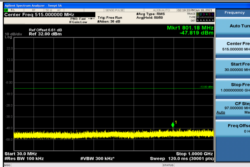
Band2-5MHz-16QAM-18900-1RB#0-30~1000MHz
