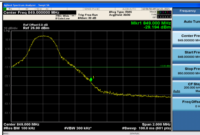
Band26-10MHz-QPSK-26990-1RB#49
