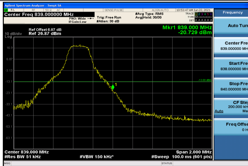
Band26-5MHz-QPSK-26915-1RB#24
