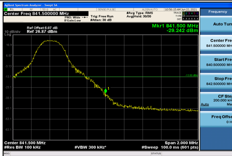
Band26-10MHz-QPSK-26915-1RB#49
