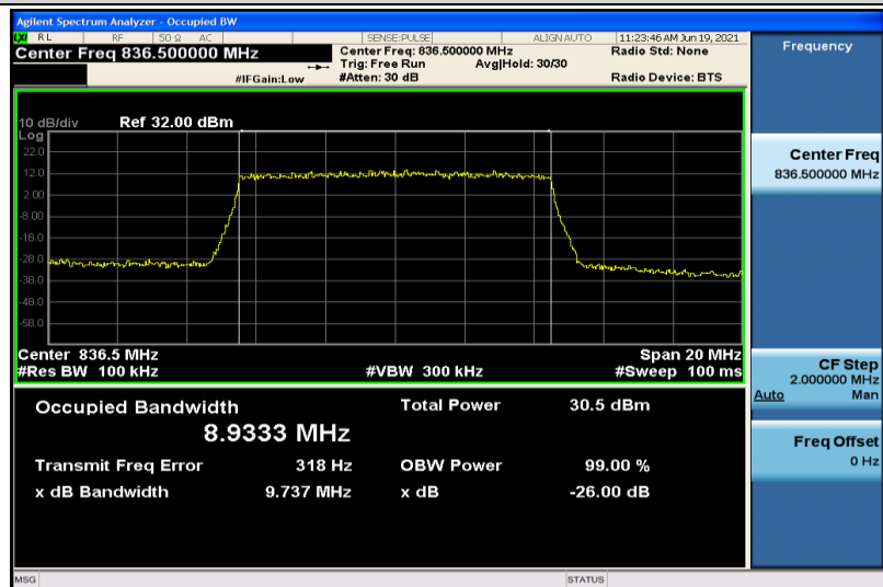
Band5-10MHz-QPSK-20525-50RB#0-8.9333
