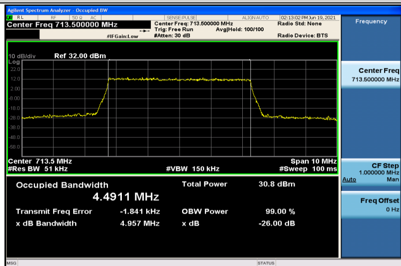
Band12-5MHz-QPSK-23155-25RB#0-4.4911
