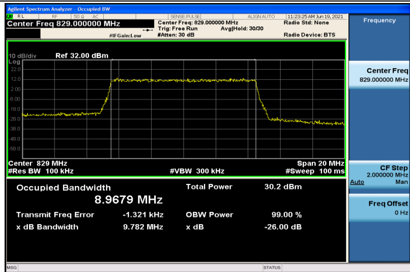
Band5-10MHz-QPSK-20450-50RB#0-8.9679
