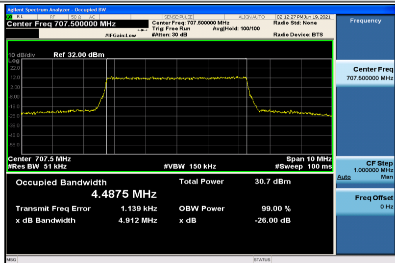
Band12-5MHz-QPSK-23095-25RB#0-4.4875
