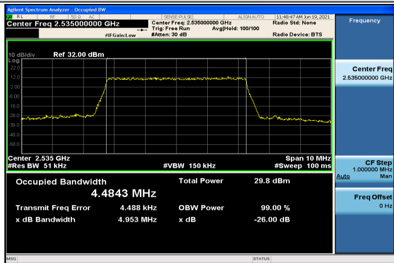
Band7-5MHz-16QAM-21100-25RB#0-4.4843
