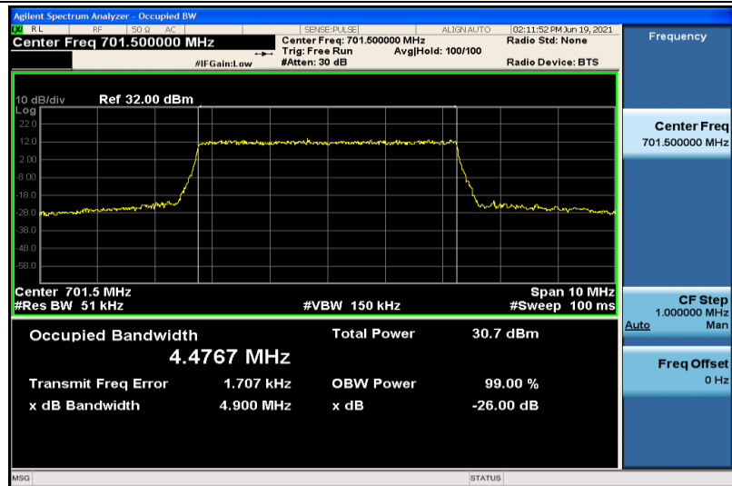
Band12-5MHz-QPSK-23035-25RB#0-4.4767
